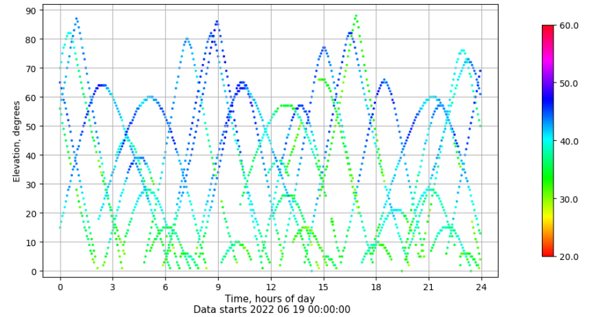
Time-elevation plot for station ALC1. Signal to Noise S1C Data file ALC100ESP_R_2022170.xtr
