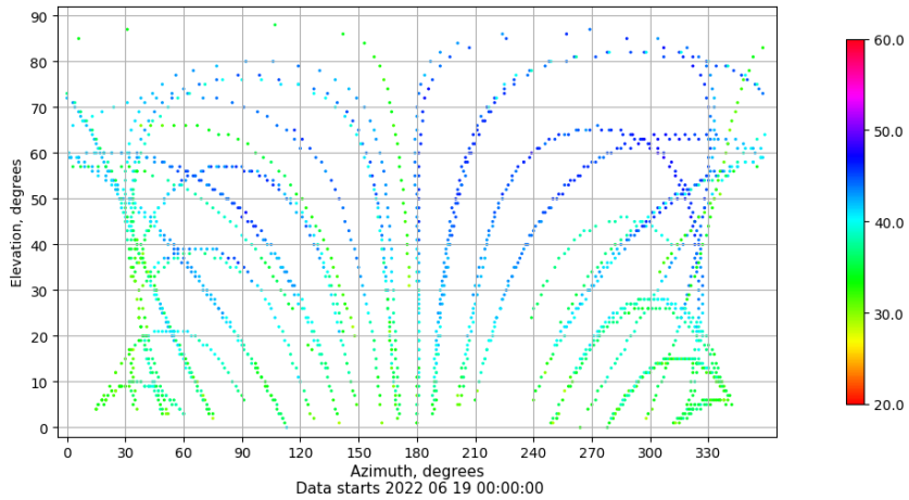
Azimuth-elevation plot for station ALC1. Signal to Noise S1C Data file ALC100ESP_R_2022170.xtr
