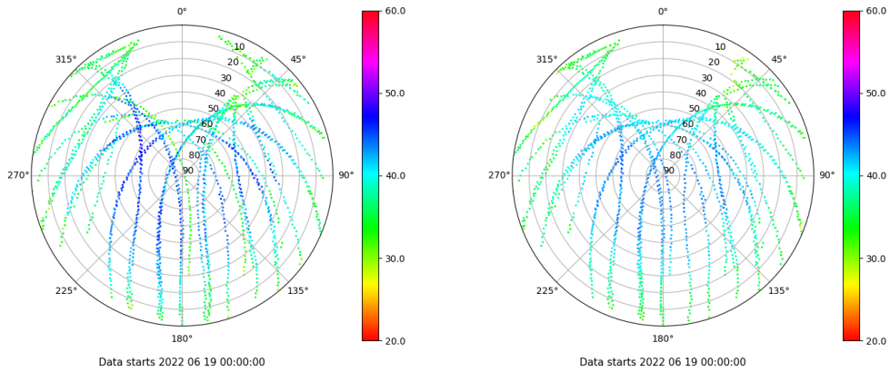
Skyplot for station ALC1. Signal to Noise S1C Data file ALC100ESP_R_2022170.xtr Skyplot for station ALC1. Signal to Noise S2C Data file ALC100ESP_R_2022170.xtr
