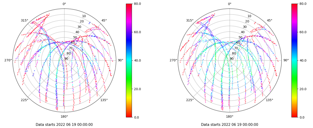
Skyplot for station ALC1. Parameter M1C Data file ALC100ESP_R_2022170.xtr Skyplot for station ALC1. Parameter M2C Data file ALC100ESP_R_2022170.xtr
