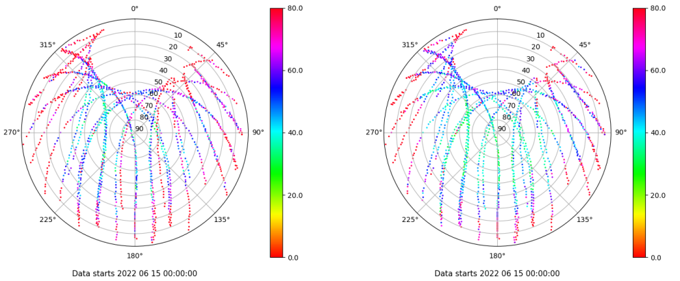
Skyplot for station ALC1. Parameter M1C Data file ALC100ESP_R_2022166.xtr Skyplot for station ALC1. Parameter M2C Data file ALC100ESP_R_2022166.xtr
