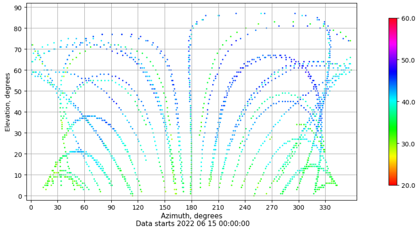
Azimuth-elevation plot for station ALC1. Signal to Noise S1C Data file ALC100ESP_R_2022166.xtr
