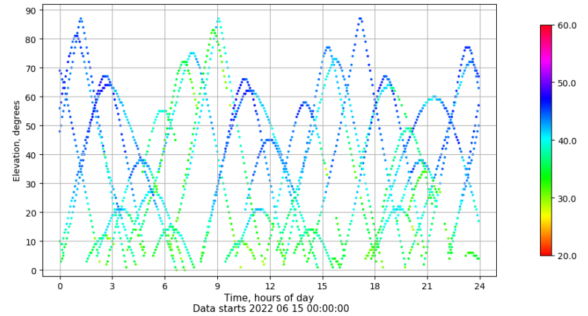
Time-elevation plot for station ALC1. Signal to Noise S1C Data file ALC100ESP_R_2022166.xtr
