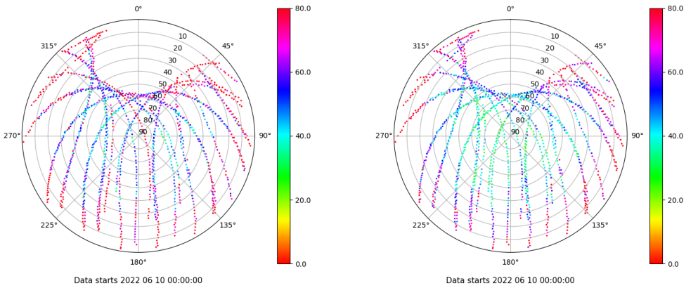
Skyplot for station ALC1. Parameter M1C Data file ALC100ESP_R_2022161.xtr Skyplot for station ALC1. Parameter M2C Data file ALC100ESP_R_2022161.xtr
