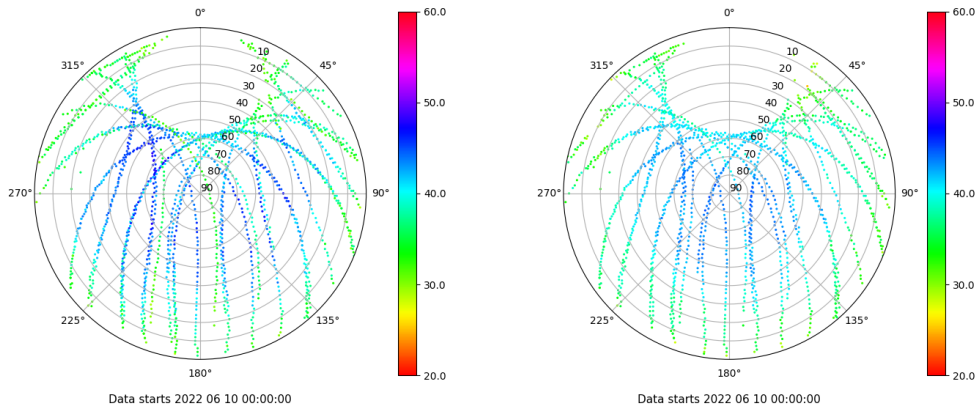
Skyplot for station ALC1. Signal to Noise S1C Data file ALC100ESP_R_2022161.xtr Skyplot for station ALC1. Signal to Noise S2C Data file ALC100ESP_R_2022161.xtr
