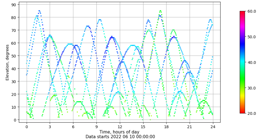
Time-elevation plot for station ALC1. Signal to Noise S1C Data file ALC100ESP_R_2022161.xtr
