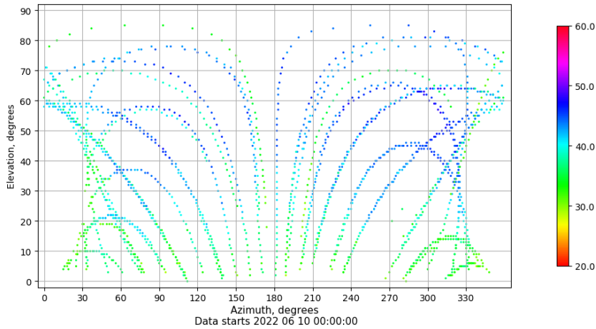
Azimuth-elevation plot for station ALC1. Signal to Noise S1C Data file ALC100ESP_R_2022161.xtr
