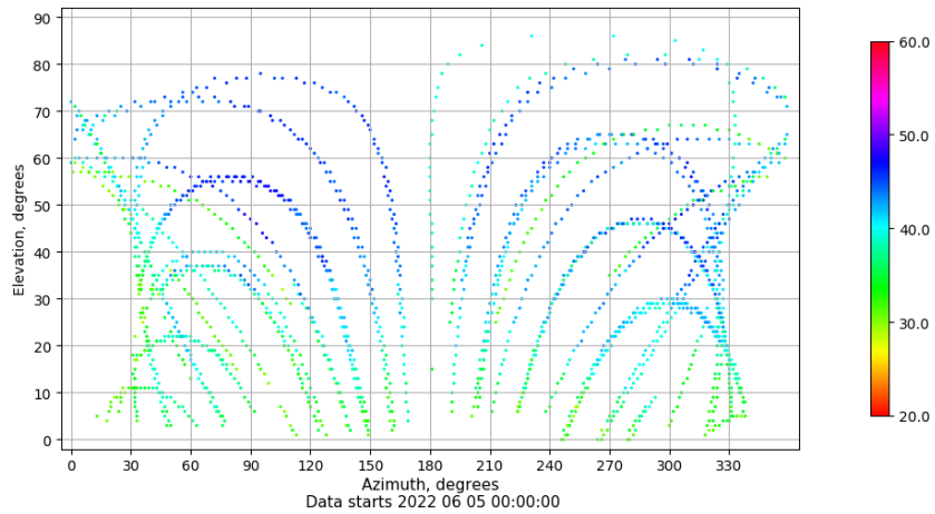
Azimuth-elevation plot for station ALC1. Signal to Noise S1C Data file ALC100ESP_R_2022156.xtr
