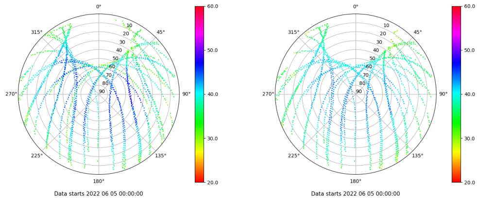
Skyplot for station ALC1. Signal to Noise S1C Data file ALC100ESP_R_2022156.xtr Skyplot for station ALC1. Signal to Noise S2C Data file ALC100ESP_R_2022156.xtr
