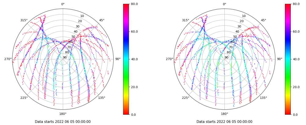
Skyplot for station ALC1. Parameter M1C Data file ALC100ESP_R_2022156.xtr Skyplot for station ALC1. Parameter M2C Data file ALC100ESP_R_2022156.xtr
