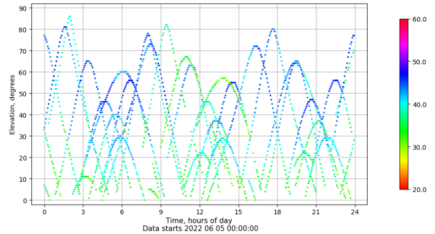
Time-elevation plot for station ALC1. Signal to Noise S1C Data file ALC100ESP_R_2022156.xtr
