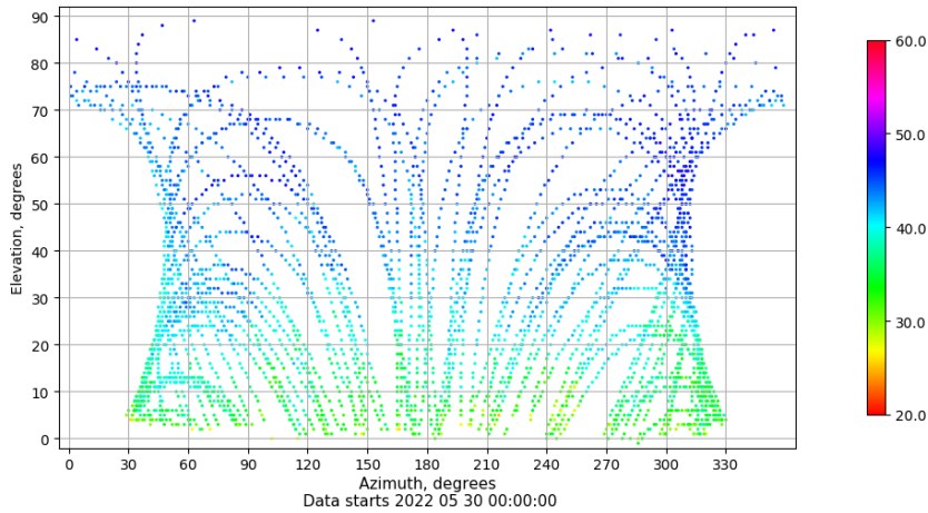
Azimuth-elevation plot for station ALC1. Signal to Noise S1C Data file ALC100ESP_R_2022150.xtr
