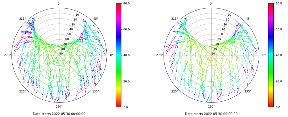
Skyplot for station ALC1. Parameter M1C Data file ALC100ESP_R_2022150.xtr Skyplot for station ALC1. Parameter M2X Data file ALC100ESP_R_2022150.xtr
