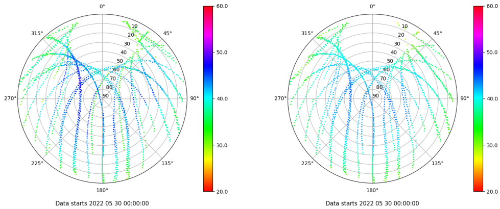
Skyplot for station ALC1. Signal to Noise S1C Data file ALC100ESP_R_2022150.xtr Skyplot for station ALC1. Signal to Noise S2C Data file ALC100ESP_R_2022150.xtr
