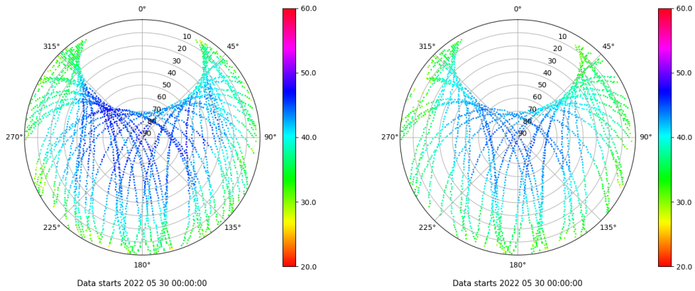
Skyplot for station ALC1. Signal to Noise S1C Data file ALC100ESP_R_2022150.xtr Skyplot for station ALC1. Signal to Noise S2X Data file ALC100ESP_R_2022150.xtr
