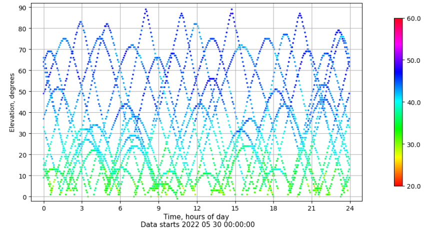
Time-elevation plot for station ALC1. Signal to Noise S1C Data file ALC100ESP_R_2022150.xtr
