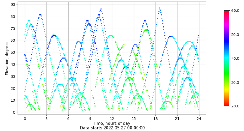
Time-elevation plot for station ALC1. Signal to Noise S1C Data file ALC100ESP_R_2022147.xtr
