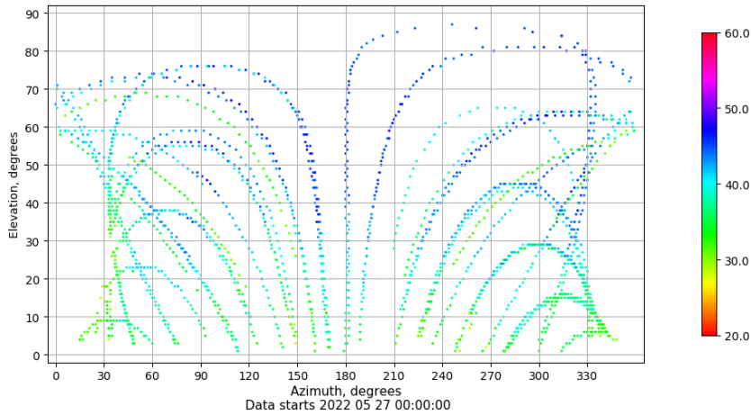
Azimuth-elevation plot for station ALC1. Signal to Noise S1C Data file ALC100ESP_R_2022147.xtr
