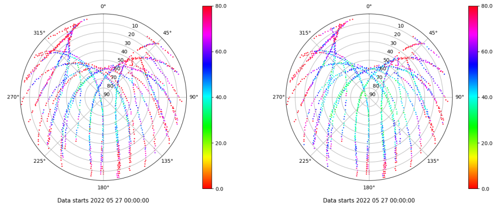
Skyplot for station ALC1. Parameter M1C Data file ALC100ESP_R_2022147.xtr Skyplot for station ALC1. Parameter M2C Data file ALC100ESP_R_2022147.xtr
