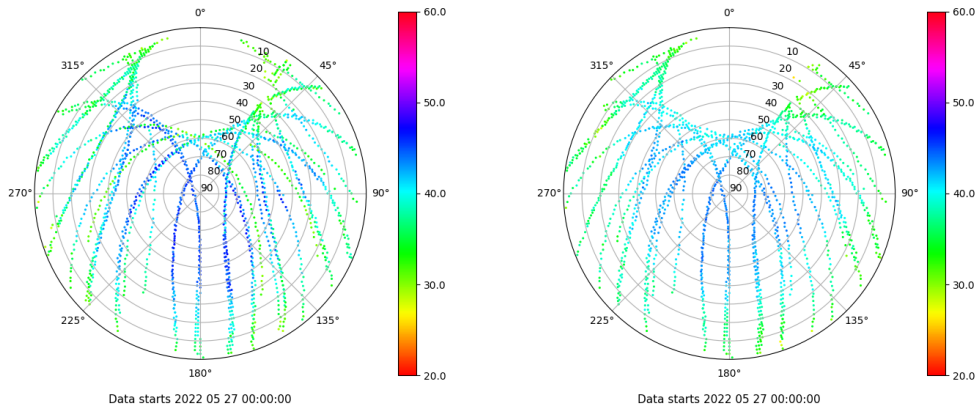
Skyplot for station ALC1. Signal to Noise S1C Data file ALC100ESP_R_2022147.xtr Skyplot for station ALC1. Signal to Noise S2C Data file ALC100ESP_R_2022147.xtr
