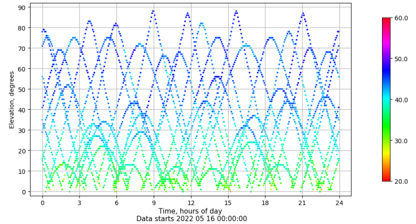
Time-elevation plot for station ALC1. Signal to Noise S1C Data file ALC100ESP_R_2022136.xtr
