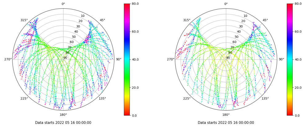
Skyplot for station ALC1. Parameter M1C Data file ALC100ESP_R_2022136.xtr Skyplot for station ALC1. Parameter M2X Data file ALC100ESP_R_2022136.xtr
