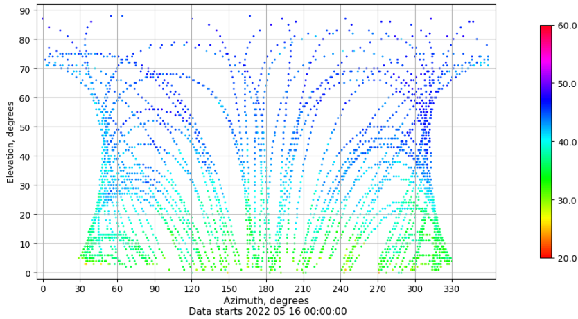
Azimuth-elevation plot for station ALC1. Signal to Noise S1C Data file ALC100ESP_R_2022136.xtr
