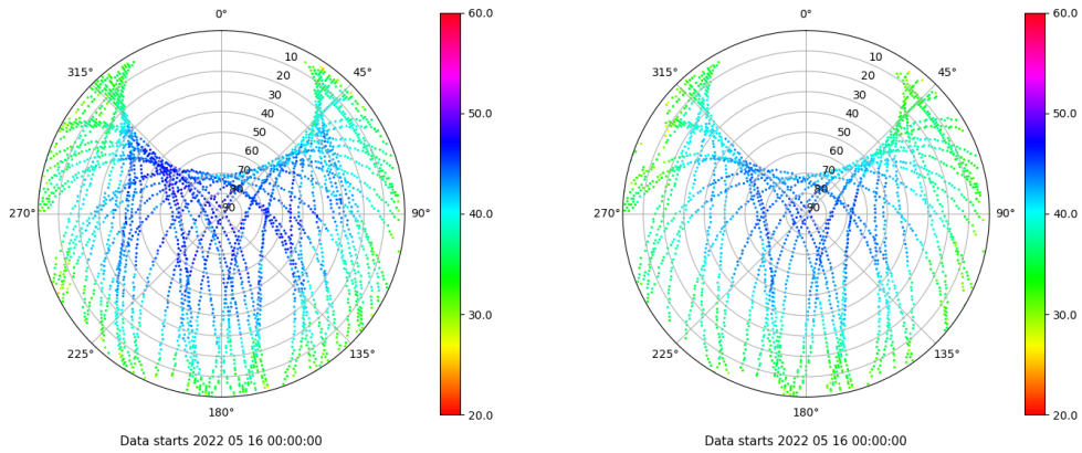
Skyplot for station ALC1. Signal to Noise S1C Data file ALC100ESP_R_2022136.xtr Skyplot for station ALC1. Signal to Noise S2X Data file ALC100ESP_R_2022136.xtr
