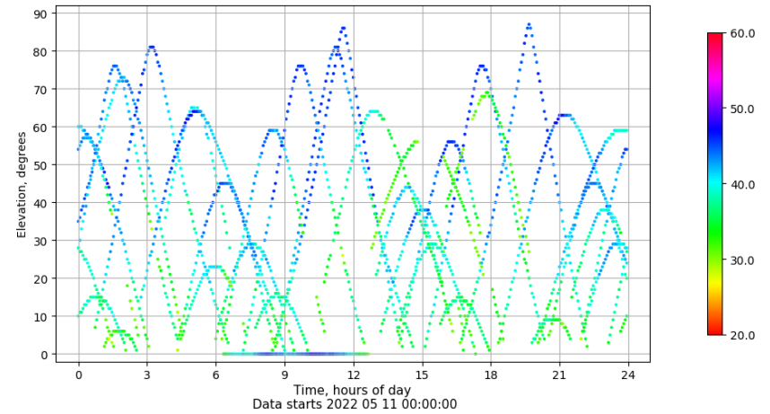
Time-elevation plot for station ALC1. Signal to Noise S1C Data file ALC100ESP_R_2022131.xtr
