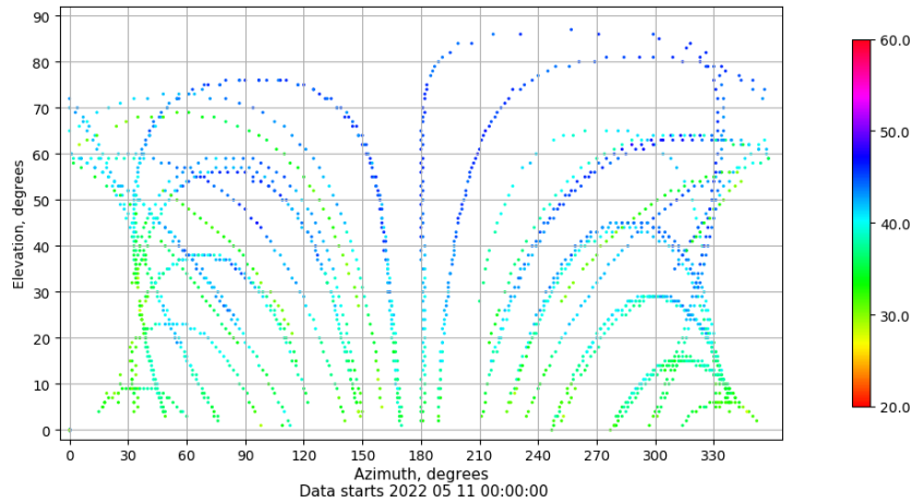
Azimuth-elevation plot for station ALC1. Signal to Noise S1C Data file ALC100ESP_R_2022131.xtr
