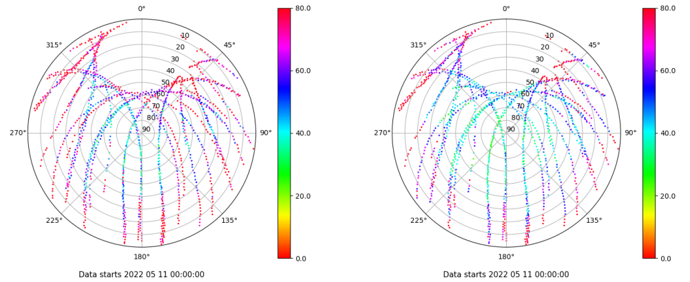
Skyplot for station ALC1. Parameter M1C Data file ALC100ESP_R_2022131.xtr Skyplot for station ALC1. Parameter M2C Data file ALC100ESP_R_2022131.xtr
