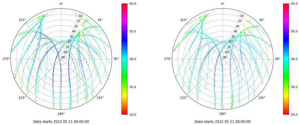
Skyplot for station ALC1. Signal to Noise S1C Data file ALC100ESP_R_2022131.xtr Skyplot for station ALC1. Signal to Noise S2C Data file ALC100ESP_R_2022131.xtr
