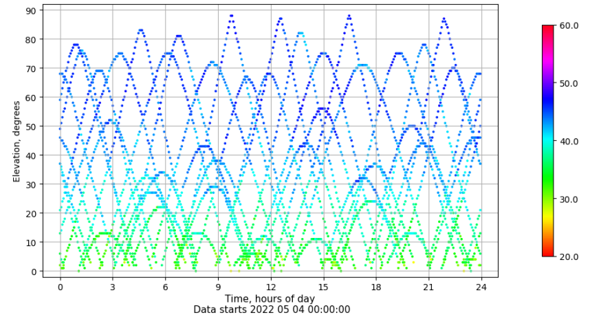
Time-elevation plot for station ALC1. Signal to Noise S1C Data file ALC100ESP_R_2022124.xtr
