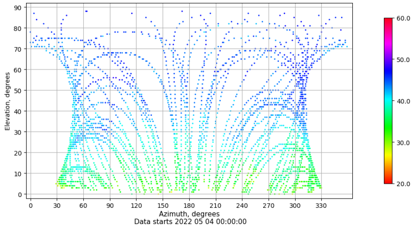
Azimuth-elevation plot for station ALC1. Signal to Noise S1C Data file ALC100ESP_R_2022124.xtr
