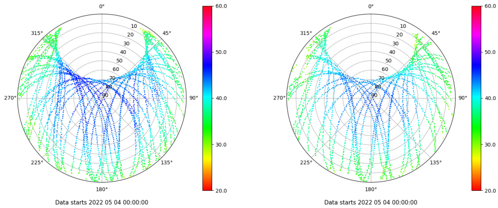
Skyplot for station ALC1. Signal to Noise S1C Data file ALC100ESP_R_2022124.xtr Skyplot for station ALC1. Signal to Noise S2X Data file ALC100ESP_R_2022124.xtr
