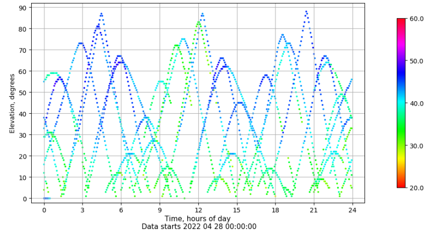
Time-elevation plot for station ALC1. Signal to Noise S1C Data file ALC100ESP_R_2022118.xtr
