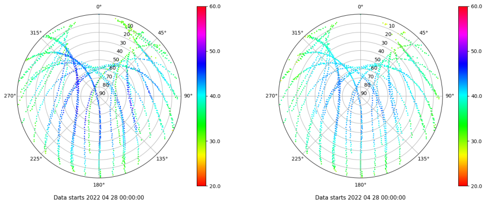
Skyplot for station ALC1. Signal to Noise S1C Data file ALC100ESP_R_2022118.xtr Skyplot for station ALC1. Signal to Noise S2C Data file ALC100ESP_R_2022118.xtr
