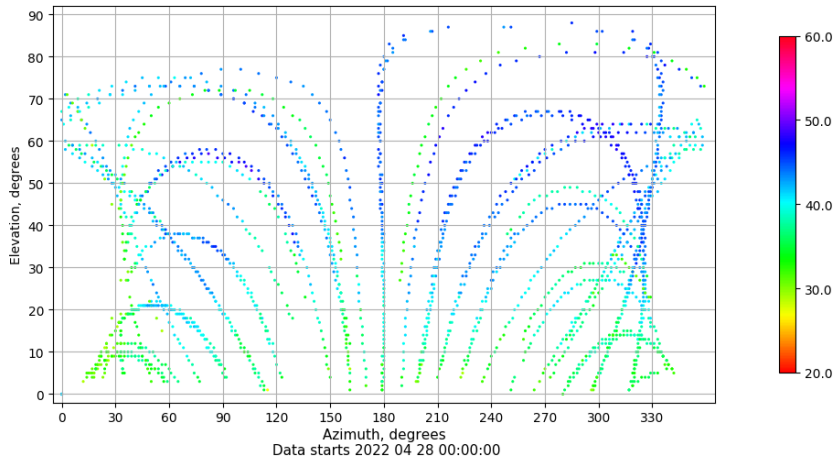
Azimuth-elevation plot for station ALC1. Signal to Noise S1C Data file ALC100ESP_R_2022118.xtr
