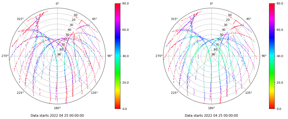
Skyplot for station ALC1. Parameter M1C Data file ALC100ESP_R_2022115.xtr Skyplot for station ALC1. Parameter M2C Data file ALC100ESP_R_2022115.xtr
