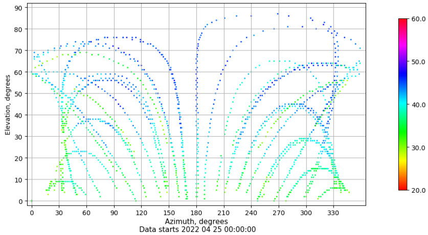
Azimuth-elevation plot for station ALC1. Signal to Noise S1C Data file ALC100ESP_R_2022115.xtr
