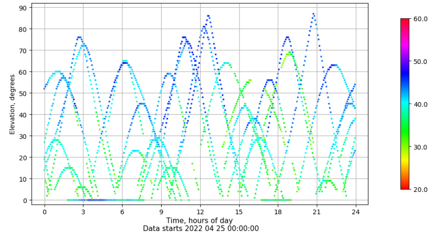
Time-elevation plot for station ALC1. Signal to Noise S1C Data file ALC100ESP_R_2022115.xtr
