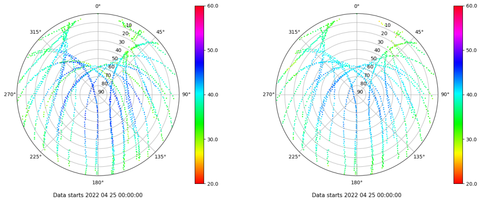
Skyplot for station ALC1. Signal to Noise S1C Data file ALC100ESP_R_2022115.xtr Skyplot for station ALC1. Signal to Noise S2C Data file ALC100ESP_R_2022115.xtr
