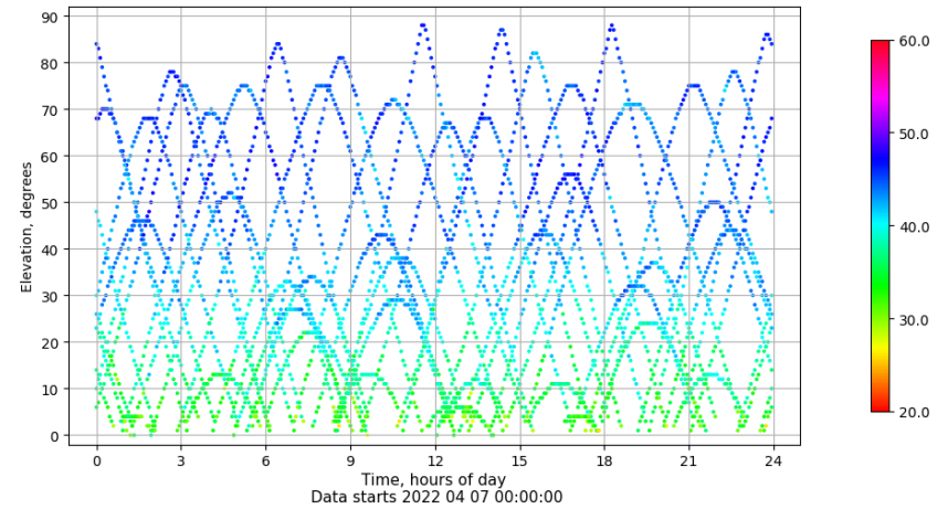
Time-elevation plot for station ALC1. Signal to Noise S1C Data file ALC100ESP_R_2022097.xtr
