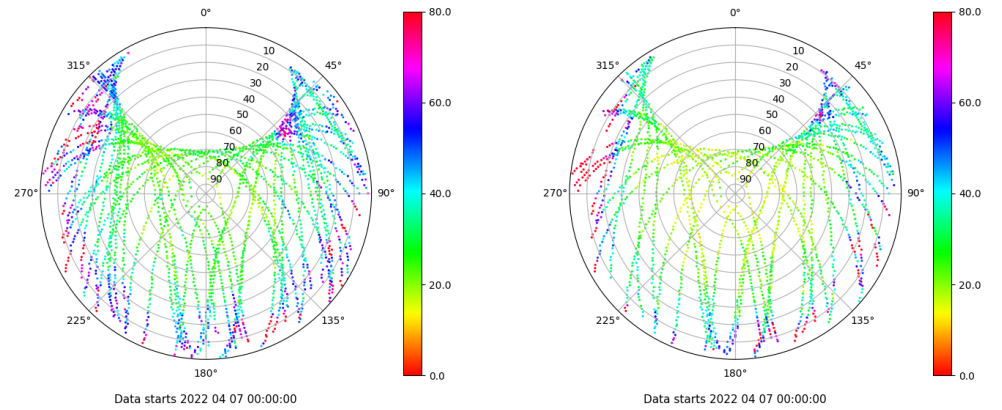
Skyplot for station ALC1. Parameter M1C Data file ALC100ESP_R_2022097.xtr Skyplot for station ALC1. Parameter M2X Data file ALC100ESP_R_2022097.xtr
