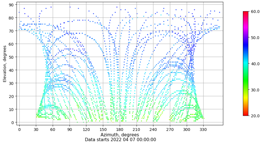
Azimuth-elevation plot for station ALC1. Signal to Noise S1C Data file ALC100ESP_R_2022097.xtr
