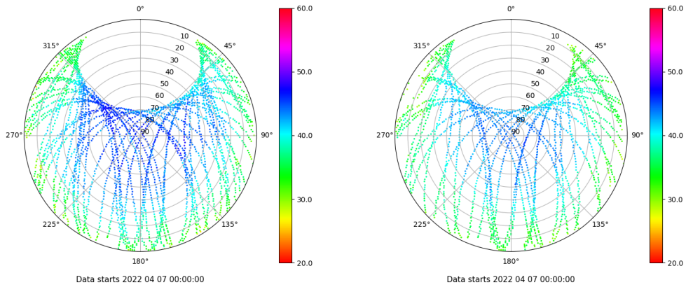
Skyplot for station ALC1. Signal to Noise S1C Data file ALC100ESP_R_2022097.xtr Skyplot for station ALC1. Signal to Noise S2X Data file ALC100ESP_R_2022097.xtr
