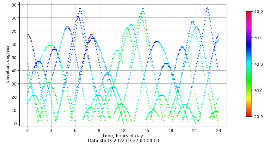
Time-elevation plot for station ALC1. Signal to Noise S1C Data file ALC100ESP_R_2022086.xtr
