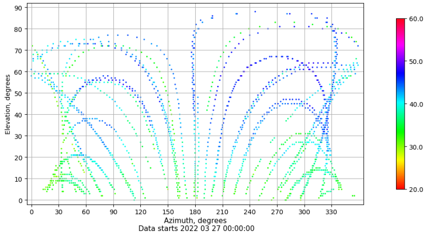
Azimuth-elevation plot for station ALC1. Signal to Noise S1C Data file ALC100ESP_R_2022086.xtr
