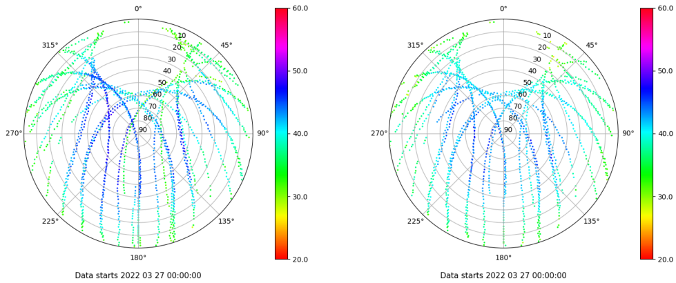
Skyplot for station ALC1. Signal to Noise S1C Data file ALC100ESP_R_2022086.xtr Skyplot for station ALC1. Signal to Noise S2C Data file ALC100ESP_R_2022086.xtr
