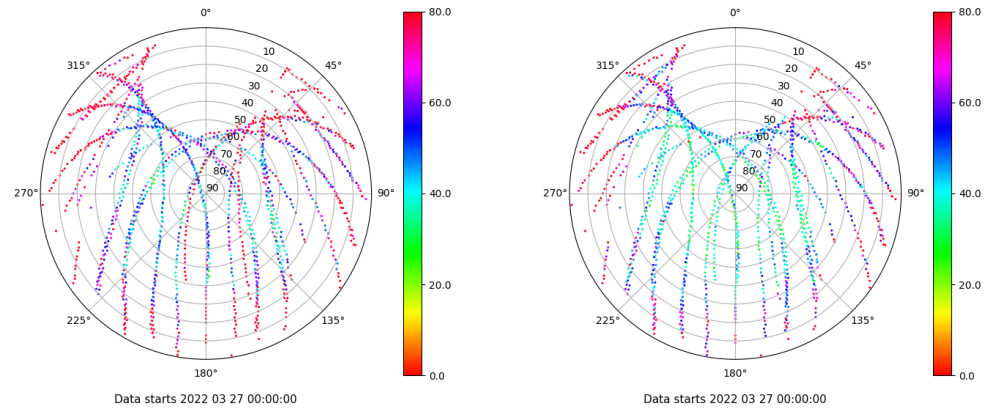
Skyplot for station ALC1. Parameter M1C Data file ALC100ESP_R_2022086.xtr Skyplot for station ALC1. Parameter M2C Data file ALC100ESP_R_2022086.xtr
