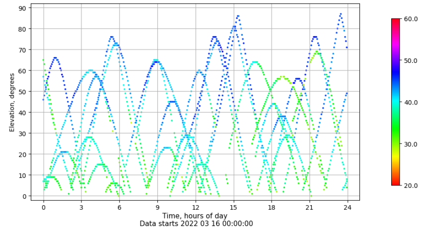
Time-elevation plot for station ALC1. Signal to Noise S1C Data file ALC100ESP_R_2022075.xtr
