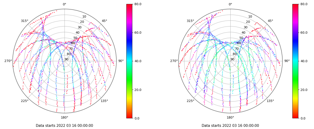
Skyplot for station ALC1. Parameter M1C Data file ALC100ESP_R_2022075.xtr Skyplot for station ALC1. Parameter M2C Data file ALC100ESP_R_2022075.xtr
