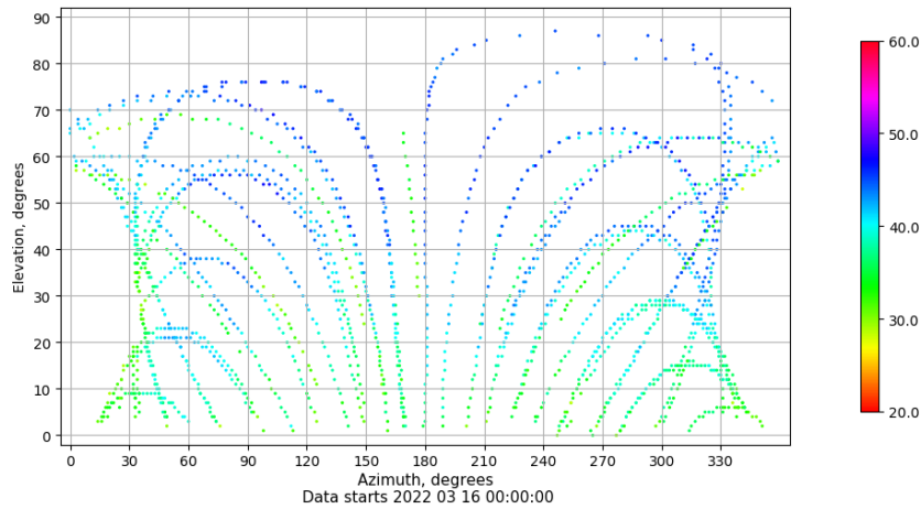
Azimuth-elevation plot for station ALC1. Signal to Noise S1C Data file ALC100ESP_R_2022075.xtr
