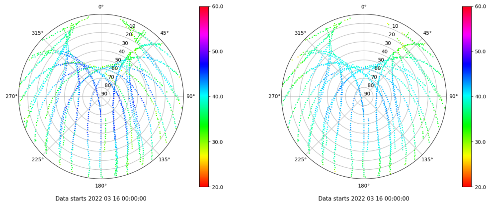
Skyplot for station ALC1. Signal to Noise S1C Data file ALC100ESP_R_2022075.xtr Skyplot for station ALC1. Signal to Noise S2C Data file ALC100ESP_R_2022075.xtr
