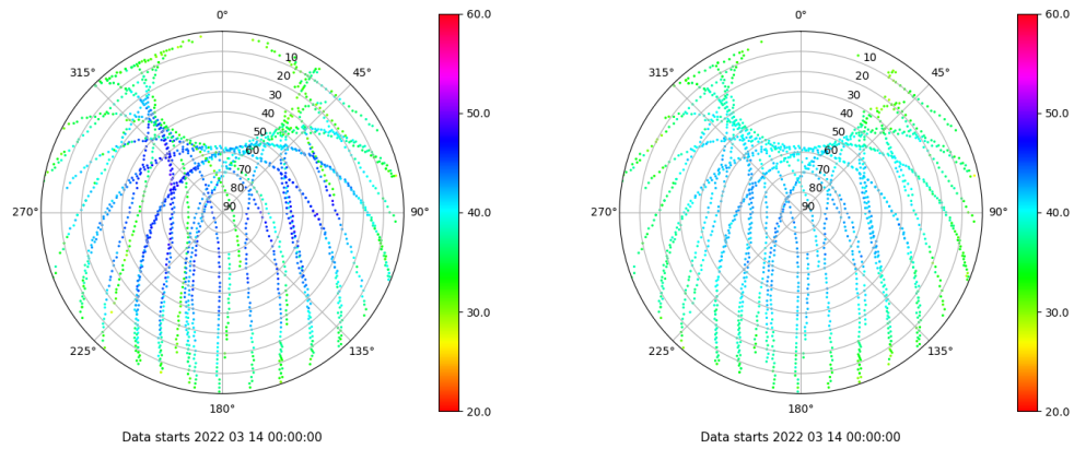
Skyplot for station ALC1. Signal to Noise S1C Data file ALC100ESP_R_2022073.xtr Skyplot for station ALC1. Signal to Noise S2C Data file ALC100ESP_R_2022073.xtr
