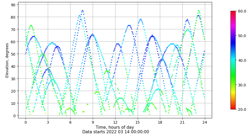
Time-elevation plot for station ALC1. Signal to Noise S1C Data file ALC100ESP_R_2022073.xtr
