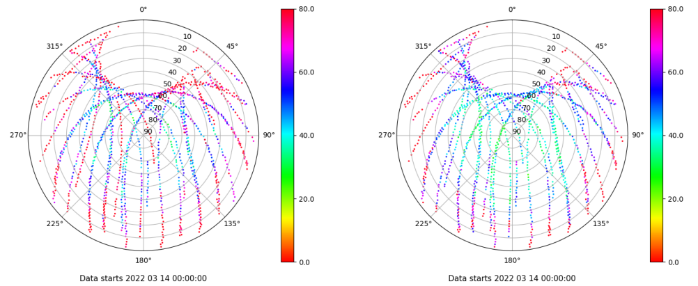
Skyplot for station ALC1. Parameter M1C Data file ALC100ESP_R_2022073.xtr Skyplot for station ALC1. Parameter M2C Data file ALC100ESP_R_2022073.xtr
