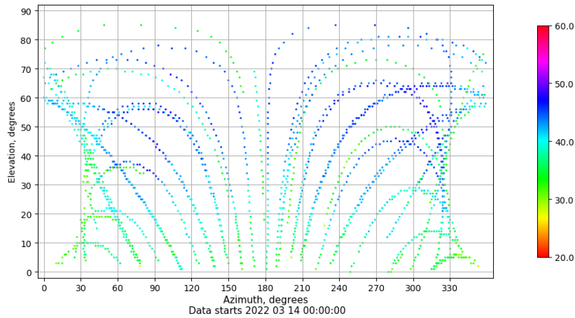
Azimuth-elevation plot for station ALC1. Signal to Noise S1C Data file ALC100ESP_R_2022073.xtr
