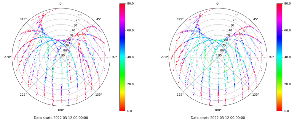
Skyplot for station ALC1. Parameter M1C Data file ALC100ESP_R_2022071.xtr Skyplot for station ALC1. Parameter M2C Data file ALC100ESP_R_2022071.xtr
