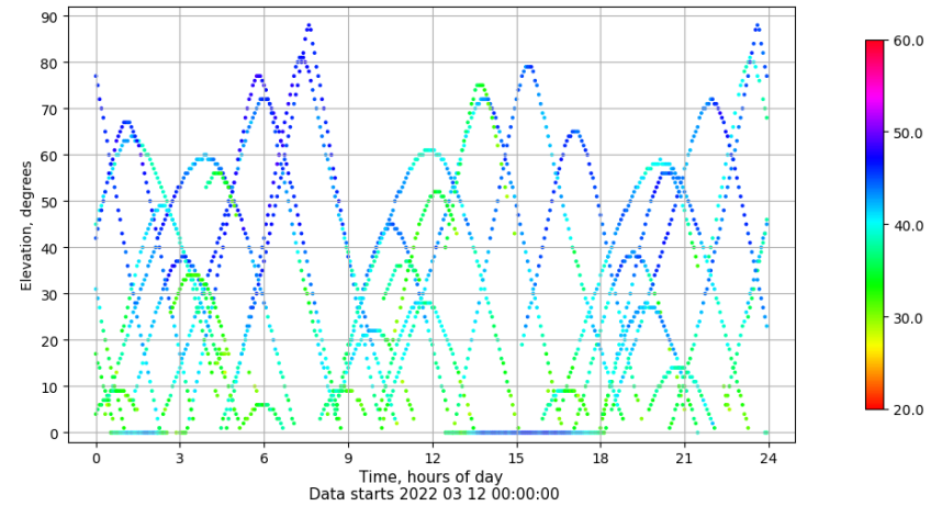
Time-elevation plot for station ALC1. Signal to Noise S1C Data file ALC100ESP_R_2022071.xtr
