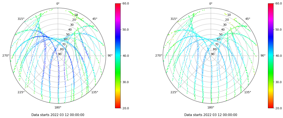
Skyplot for station ALC1. Signal to Noise S1C Data file ALC100ESP_R_2022071.xtr Skyplot for station ALC1. Signal to Noise S2C Data file ALC100ESP_R_2022071.xtr
