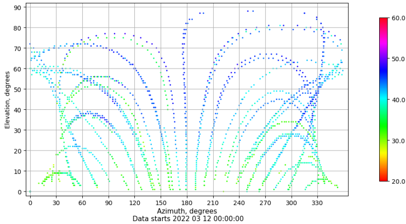
Azimuth-elevation plot for station ALC1. Signal to Noise S1C Data file ALC100ESP_R_2022071.xtr
