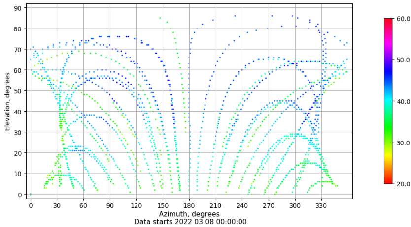
Azimuth-elevation plot for station ALC1. Signal to Noise S1C Data file ALC100ESP_R_2022067.xtr
