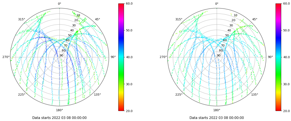
Skyplot for station ALC1. Signal to Noise S1C Data file ALC100ESP_R_2022067.xtr Skyplot for station ALC1. Signal to Noise S2C Data file ALC100ESP_R_2022067.xtr
