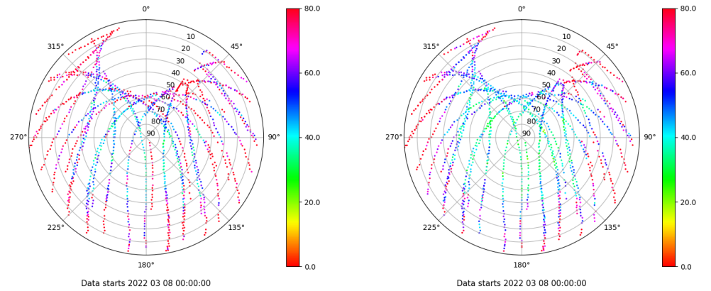
Skyplot for station ALC1. Parameter M1C Data file ALC100ESP_R_2022067.xtr Skyplot for station ALC1. Parameter M2C Data file ALC100ESP_R_2022067.xtr
