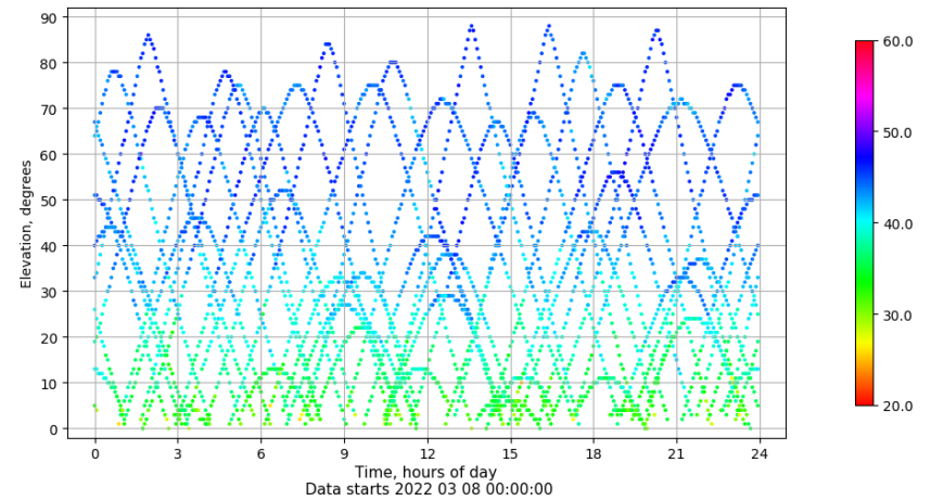
Time-elevation plot for station ALC1. Signal to Noise S1C Data file ALC100ESP_R_2022067.xtr
