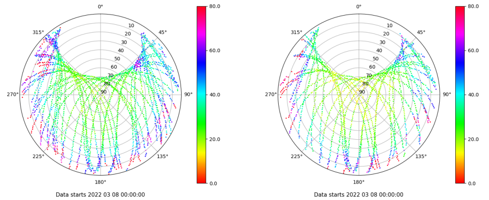
Skyplot for station ALC1. Parameter M1C Data file ALC100ESP_R_2022067.xtr Skyplot for station ALC1. Parameter M2X Data file ALC100ESP_R_2022067.xtr
