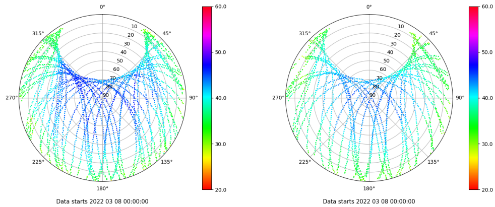
Skyplot for station ALC1. Signal to Noise S1C Data file ALC100ESP_R_2022067.xtr Skyplot for station ALC1. Signal to Noise S2X Data file ALC100ESP_R_2022067.xtr
