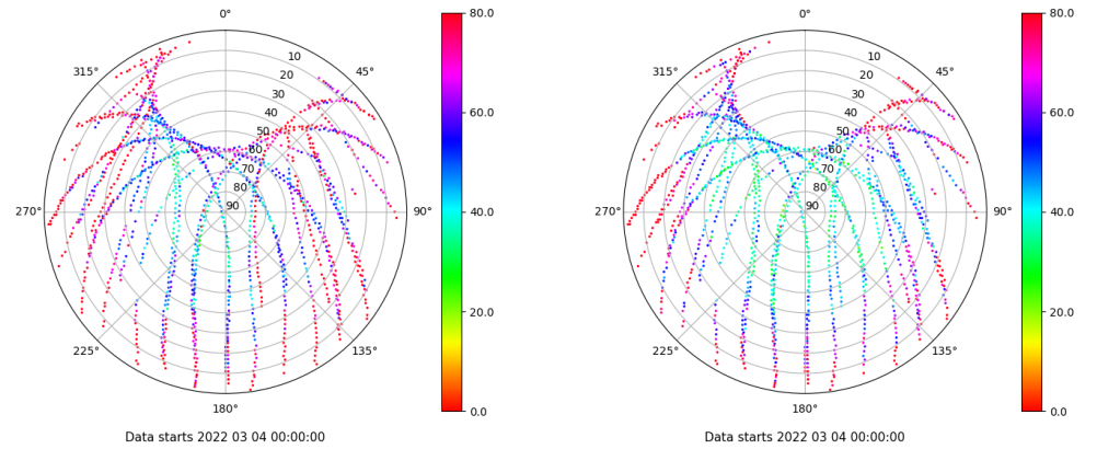
Skyplot for station ALC1. Parameter M1C Data file ALC100ESP_R_2022063.xtr Skyplot for station ALC1. Parameter M2C Data file ALC100ESP_R_2022063.xtr
