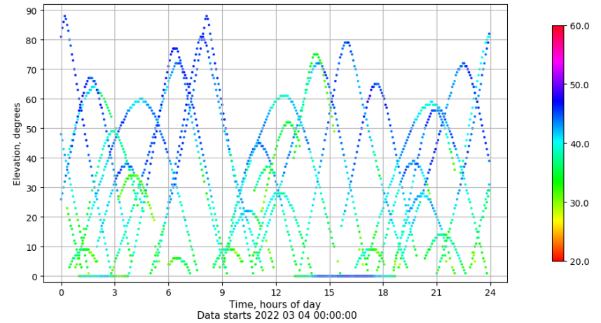
Time-elevation plot for station ALC1. Signal to Noise S1C Data file ALC100ESP_R_2022063.xtr
