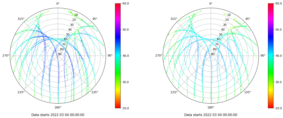
Skyplot for station ALC1. Signal to Noise S1C Data file ALC100ESP_R_2022063.xtr Skyplot for station ALC1. Signal to Noise S2C Data file ALC100ESP_R_2022063.xtr
