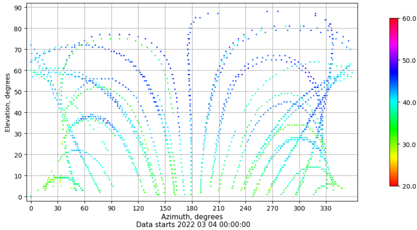
Azimuth-elevation plot for station ALC1. Signal to Noise S1C Data file ALC100ESP_R_2022063.xtr
