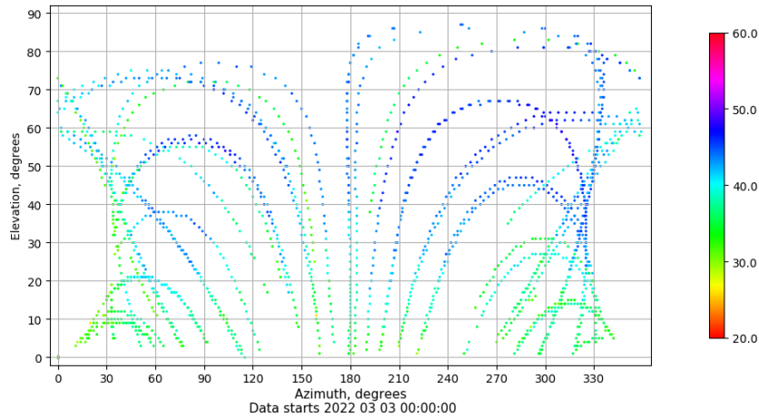
Azimuth-elevation plot for station ALC1. Signal to Noise S1C Data file ALC100ESP_R_2022062.xtr
