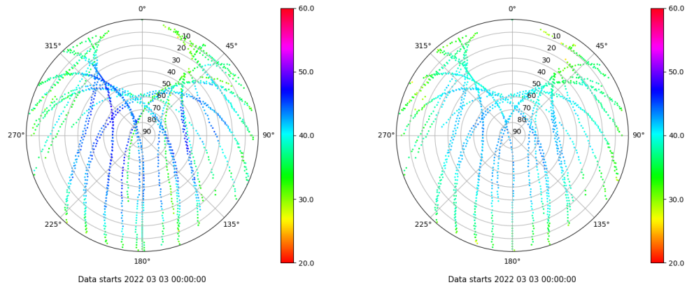
Skyplot for station ALC1. Signal to Noise S1C Data file ALC100ESP_R_2022062.xtr Skyplot for station ALC1. Signal to Noise S2C Data file ALC100ESP_R_2022062.xtr
