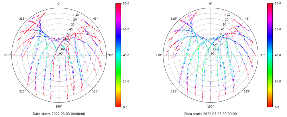
Skyplot for station ALC1. Parameter M1C Data file ALC100ESP_R_2022062.xtr Skyplot for station ALC1. Parameter M2C Data file ALC100ESP_R_2022062.xtr
