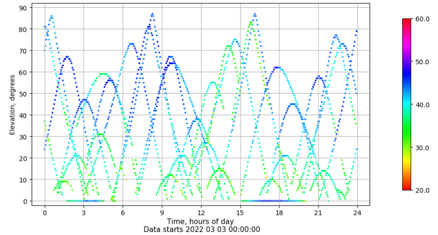
Time-elevation plot for station ALC1. Signal to Noise S1C Data file ALC100ESP_R_2022062.xtr
