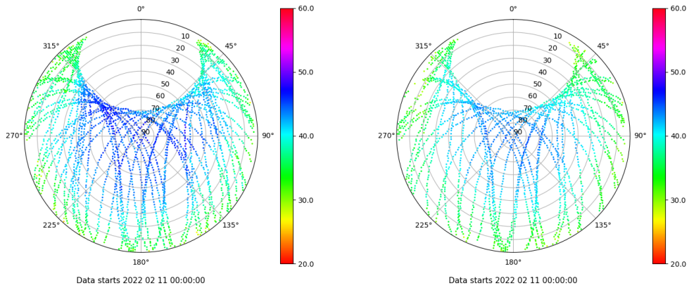
Skyplot for station ALC1. Signal to Noise S1C Data file ALC100ESP_R_2022042.xtr Skyplot for station ALC1. Signal to Noise S2X Data file ALC100ESP_R_2022042.xtr
