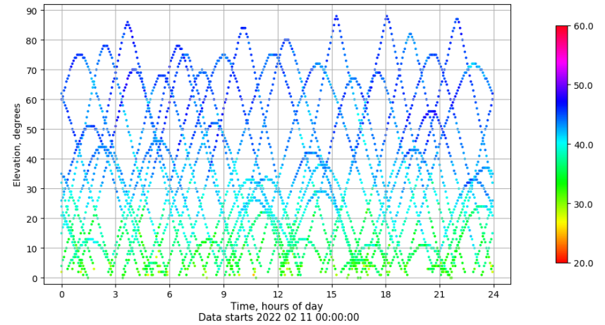
Time-elevation plot for station ALC1. Signal to Noise S1C Data file ALC100ESP_R_2022042.xtr
