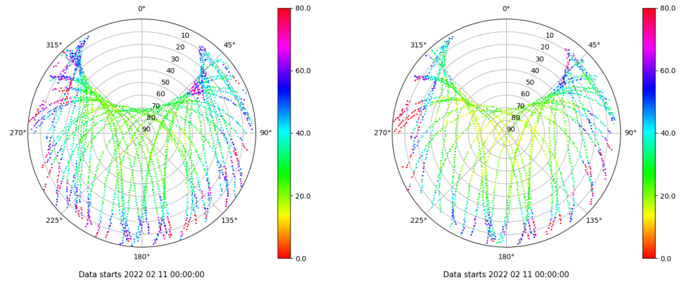
Skyplot for station ALC1. Parameter M1C Data file ALC100ESP_R_2022042.xtr Skyplot for station ALC1. Parameter M2X Data file ALC100ESP_R_2022042.xtr
