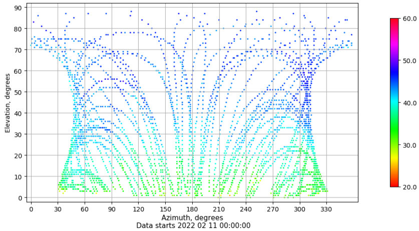
Azimuth-elevation plot for station ALC1. Signal to Noise S1C Data file ALC100ESP_R_2022042.xtr
