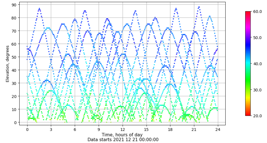
Time-elevation plot for station ALC1. Signal to Noise S1C Data file ALC100ESP_R_2021355.xtr
