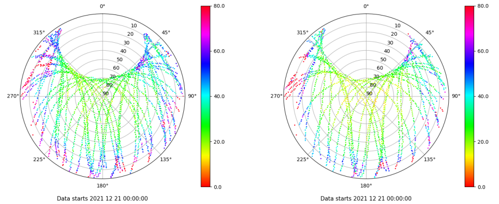
Skyplot for station ALC1. Parameter M1C Data file ALC100ESP_R_2021355.xtr Skyplot for station ALC1. Parameter M2X Data file ALC100ESP_R_2021355.xtr
