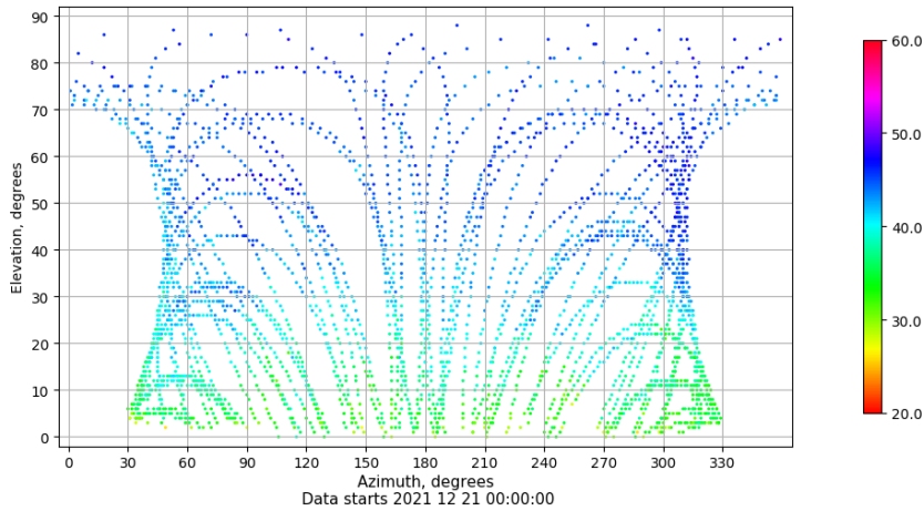
Azimuth-elevation plot for station ALC1. Signal to Noise S1C Data file ALC100ESP_R_2021355.xtr
