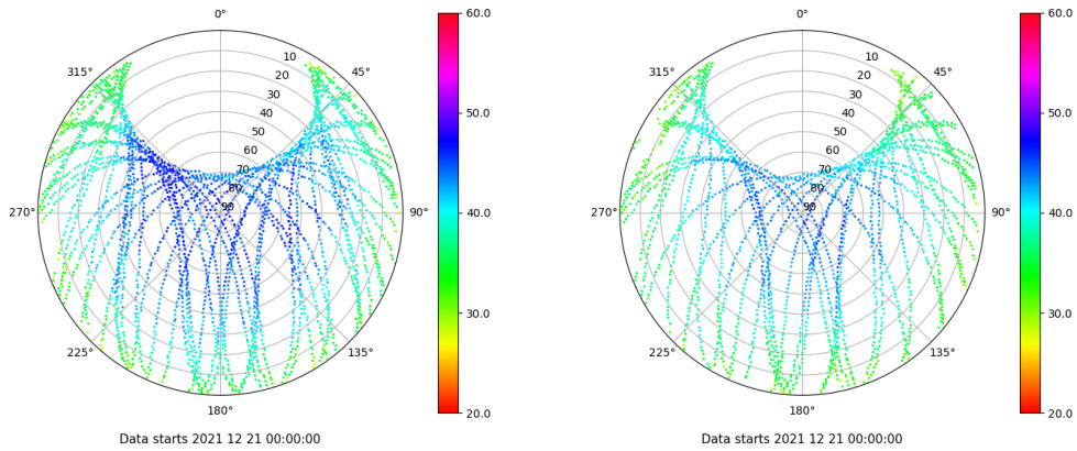
Skyplot for station ALC1. Signal to Noise S1C Data file ALC100ESP_R_2021355.xtr Skyplot for station ALC1. Signal to Noise S2X Data file ALC100ESP_R_2021355.xtr
