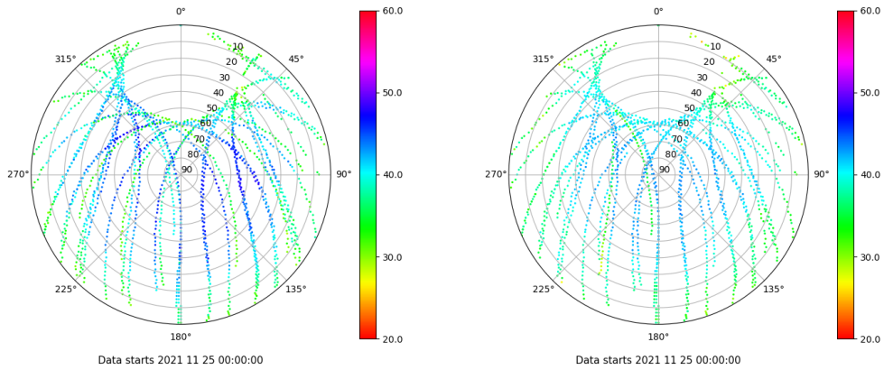
Skyplot for station ALC1. Signal to Noise S1C Data file ALC100ESP_R_2021329.xtr Skyplot for station ALC1. Signal to Noise S2C Data file ALC100ESP_R_2021329.xtr
