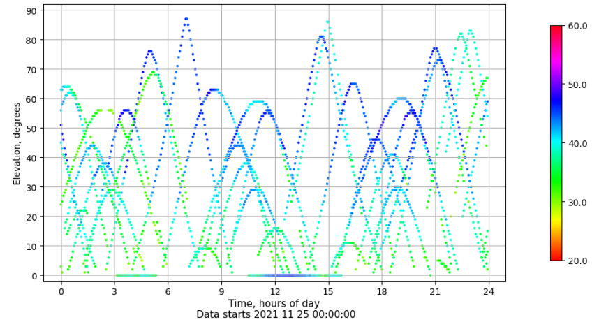
Time-elevation plot for station ALC1. Signal to Noise S1C Data file ALC100ESP_R_2021329.xtr
