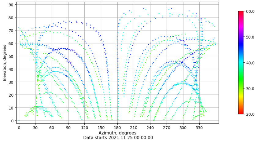
Azimuth-elevation plot for station ALC1. Signal to Noise S1C Data file ALC100ESP_R_2021329.xtr
