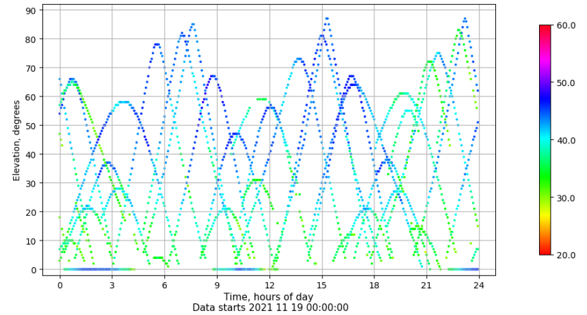
Time-elevation plot for station ALC1. Signal to Noise S1C Data file ALC100ESP_R_2021323.xtr
