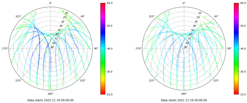
Skyplot for station ALC1. Signal to Noise S1C Data file ALC100ESP_R_2021323.xtr Skyplot for station ALC1. Signal to Noise S2C Data file ALC100ESP_R_2021323.xtr
