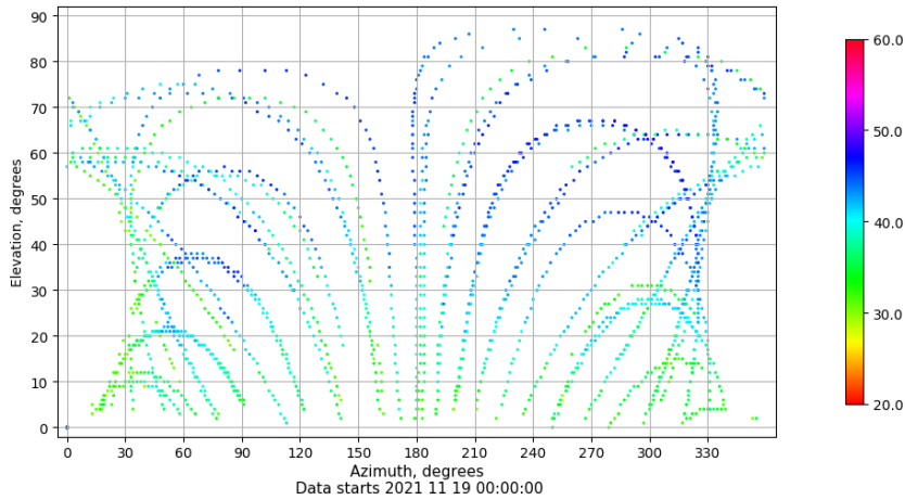
Azimuth-elevation plot for station ALC1. Signal to Noise S1C Data file ALC100ESP_R_2021323.xtr
