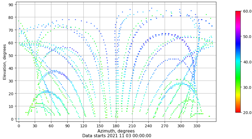
Azimuth-elevation plot for station ALC1. Signal to Noise S1C Data file ALC100ESP_R_2021307.xtr
