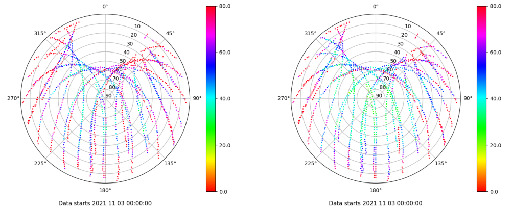
Skyplot for station ALC1. Parameter M1C Data file ALC100ESP_R_2021307.xtr Skyplot for station ALC1. Parameter M2C Data file ALC100ESP_R_2021307.xtr
