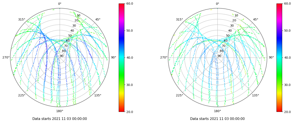
Skyplot for station ALC1. Signal to Noise S1C Data file ALC100ESP_R_2021307.xtr Skyplot for station ALC1. Signal to Noise S2C Data file ALC100ESP_R_2021307.xtr
