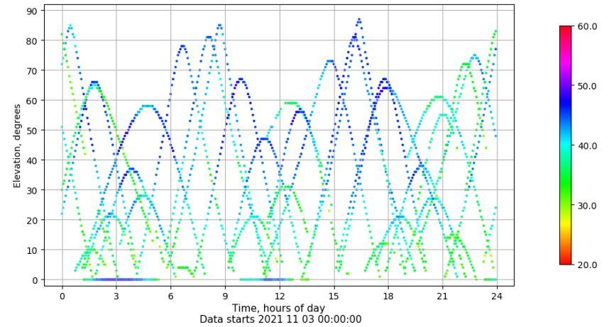
Time-elevation plot for station ALC1. Signal to Noise S1C Data file ALC100ESP_R_2021307.xtr
