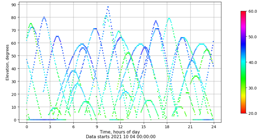
Time-elevation plot for station ALC1. Signal to Noise S1C Data file ALC100ESP_R_2021277.xtr
