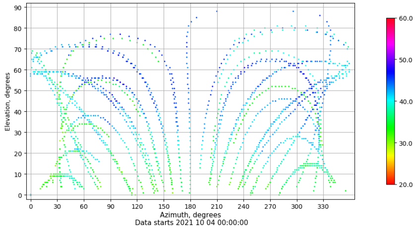
Azimuth-elevation plot for station ALC1. Signal to Noise S1C Data file ALC100ESP_R_2021277.xtr
