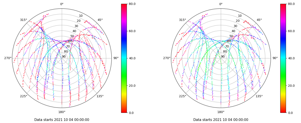
Skyplot for station ALC1. Parameter M1C Data file ALC100ESP_R_2021277.xtr Skyplot for station ALC1. Parameter M2C Data file ALC100ESP_R_2021277.xtr
