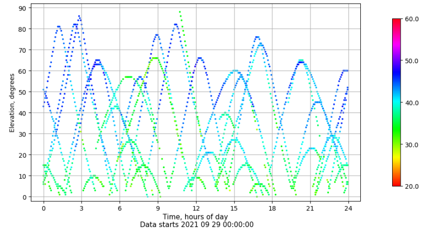
Time-elevation plot for station ALC1. Signal to Noise S1C Data file ALC100ESP_R_2021272.xtr
