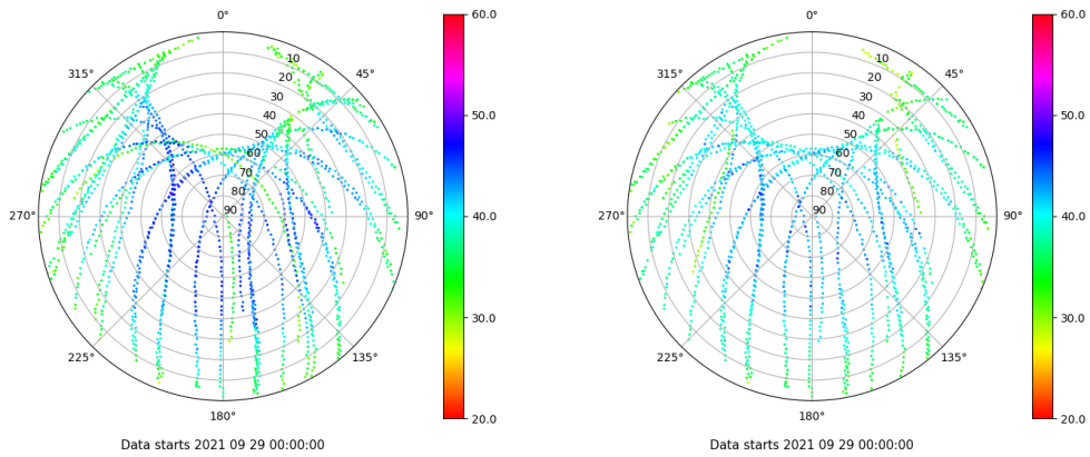
Skyplot for station ALC1. Signal to Noise S1C Data file ALC100ESP_R_2021272.xtr Skyplot for station ALC1. Signal to Noise S2C Data file ALC100ESP_R_2021272.xtr
