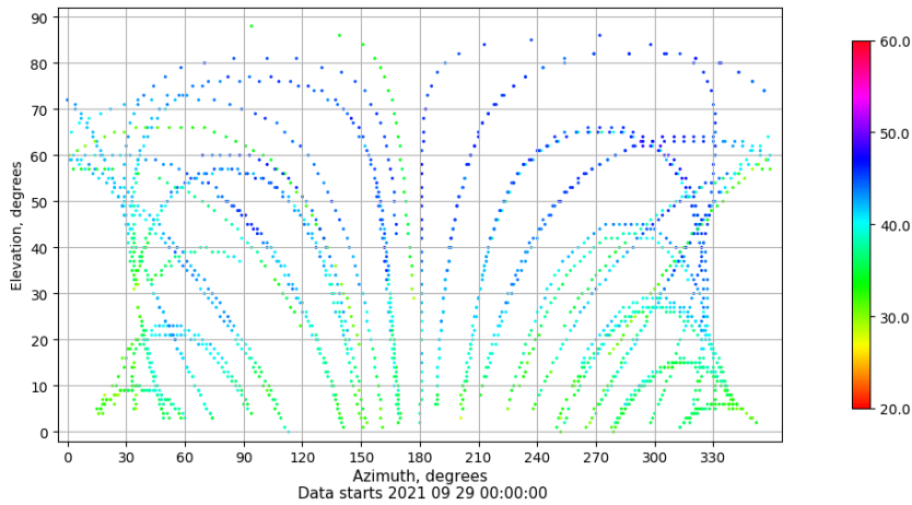
Azimuth-elevation plot for station ALC1. Signal to Noise S1C Data file ALC100ESP_R_2021272.xtr
