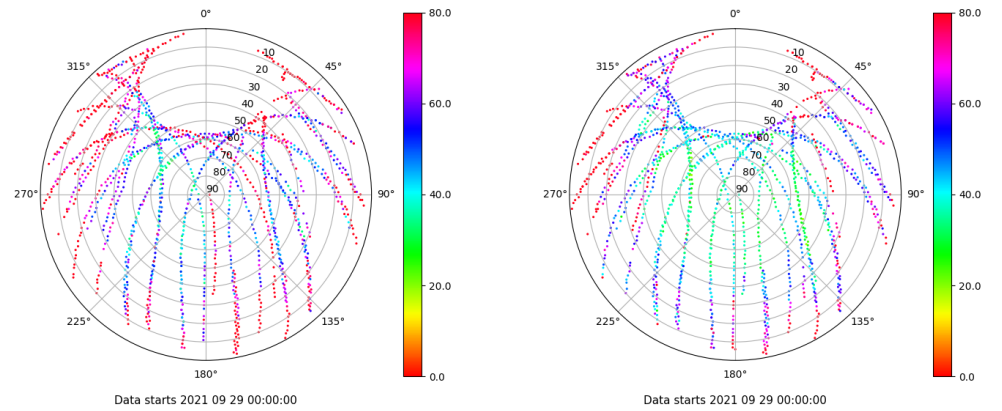
Skyplot for station ALC1. Parameter M1C Data file ALC100ESP_R_2021272.xtr Skyplot for station ALC1. Parameter M2C Data file ALC100ESP_R_2021272.xtr
