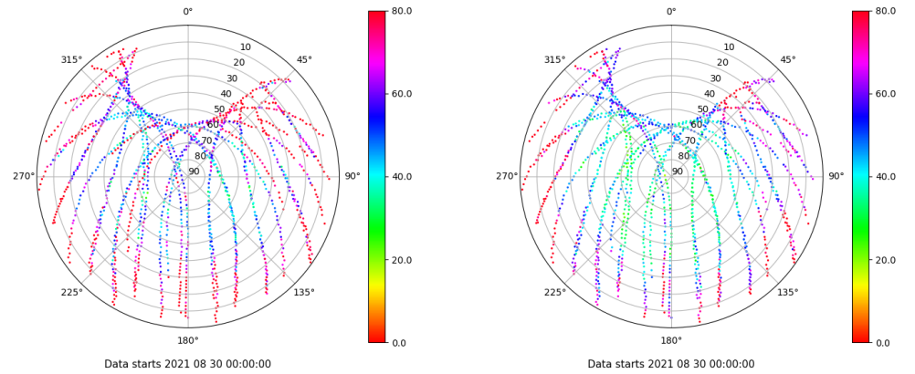
Skyplot for station ALC1. Parameter M1C Data file ALC100ESP_R_2021242.xtr Skyplot for station ALC1. Parameter M2C Data file ALC100ESP_R_2021242.xtr
