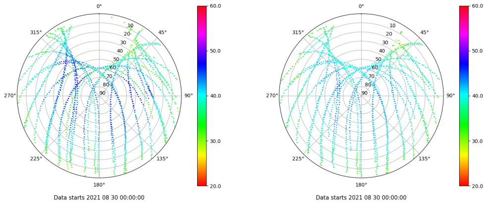
Skyplot for station ALC1. Signal to Noise S1C Data file ALC100ESP_R_2021242.xtr Skyplot for station ALC1. Signal to Noise S2C Data file ALC100ESP_R_2021242.xtr
