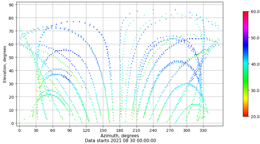
Azimuth-elevation plot for station ALC1. Signal to Noise S1C Data file ALC100ESP_R_2021242.xtr
