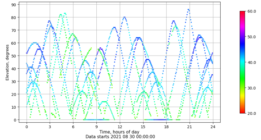
Time-elevation plot for station ALC1. Signal to Noise S1C Data file ALC100ESP_R_2021242.xtr
