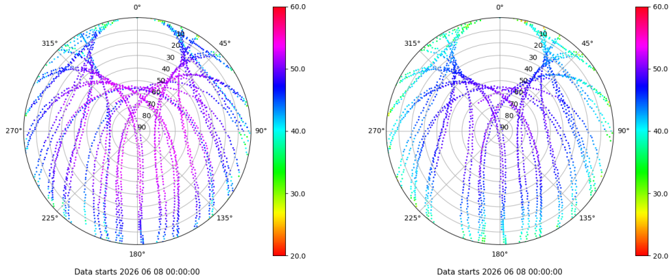
Skyplot for station ALBA. Signal to Noise S1C Data file ALBA00ESP_R_2026159.xtr Skyplot for station ALBA. Signal to Noise S2C Data file ALBA00ESP_R_2026159.xtr
