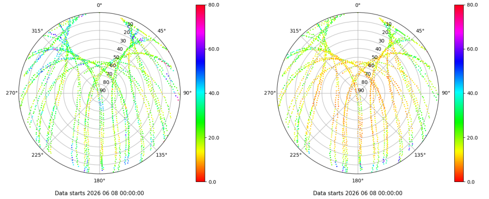
Skyplot for station ALBA. Parameter M1C Data file ALBA00ESP_R_2026159.xtr Skyplot for station ALBA. Parameter M2C Data file ALBA00ESP_R_2026159.xtr
