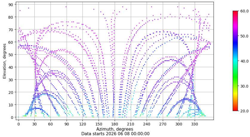
Azimuth-elevation plot for station ALBA. Signal to Noise S1C Data file ALBA00ESP_R_2026159.xtr
