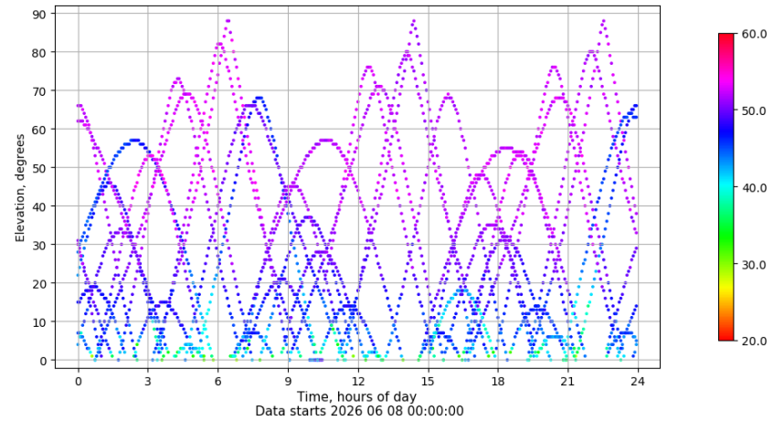
Time-elevation plot for station ALBA. Signal to Noise S1C Data file ALBA00ESP_R_2026159.xtr
