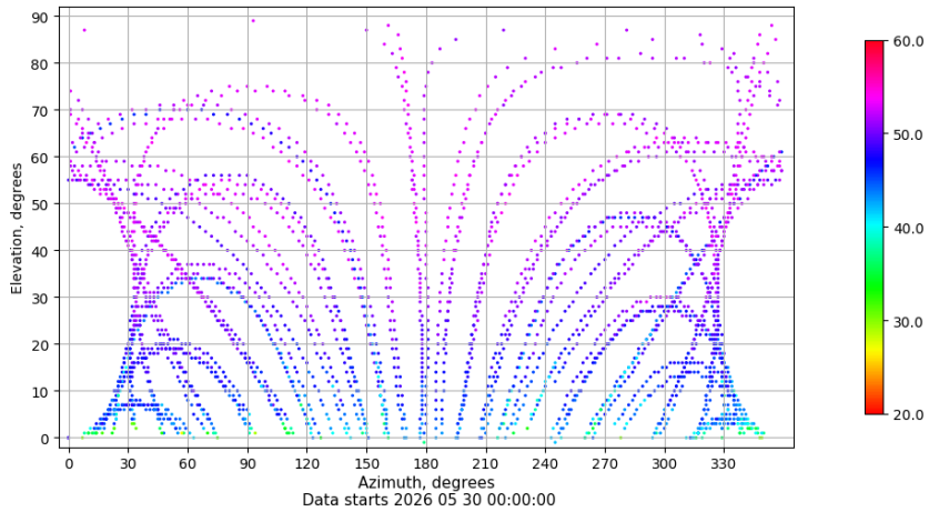
Azimuth-elevation plot for station ALBA. Signal to Noise S1C Data file ALBA00ESP_R_2026150.xtr
