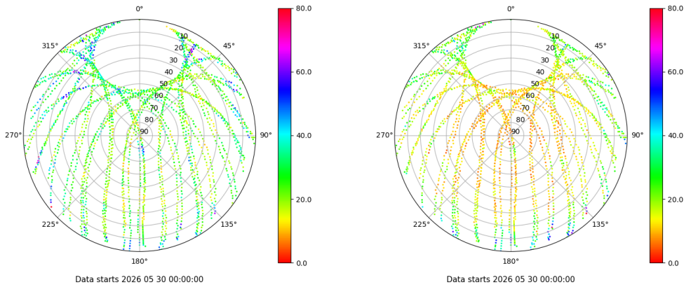
Skyplot for station ALBA. Parameter M1C Data file ALBA00ESP_R_2026150.xtr Skyplot for station ALBA. Parameter M2C Data file ALBA00ESP_R_2026150.xtr
