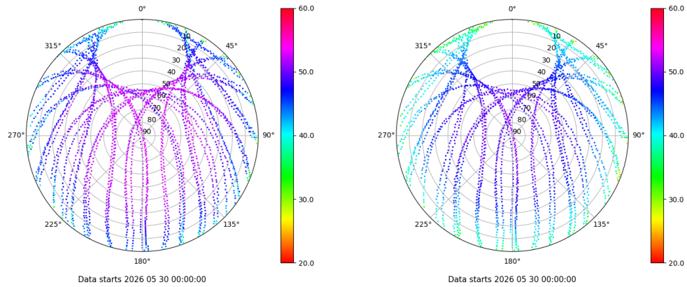
Skyplot for station ALBA. Signal to Noise S1C Data file ALBA00ESP_R_2026150.xtr Skyplot for station ALBA. Signal to Noise S2C Data file ALBA00ESP_R_2026150.xtr
