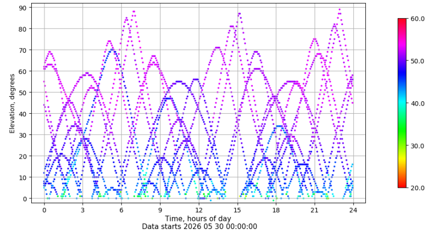
Time-elevation plot for station ALBA. Signal to Noise S1C Data file ALBA00ESP_R_2026150.xtr
