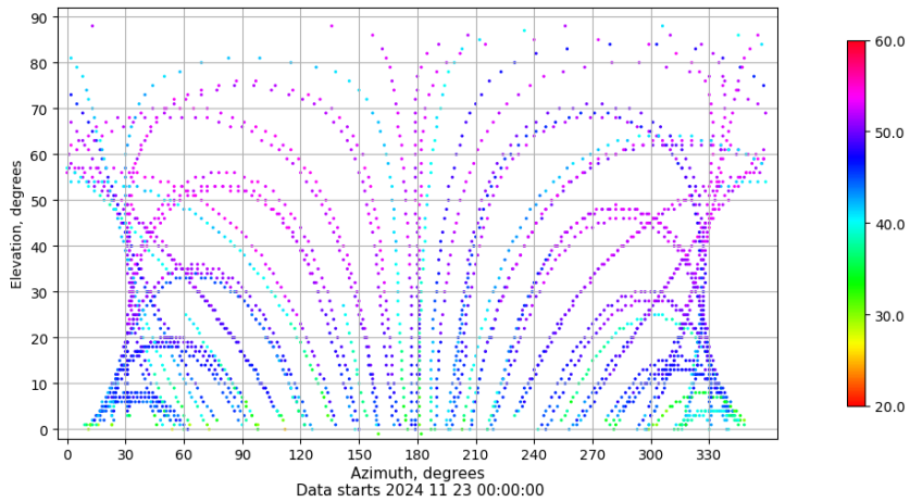
Azimuth-elevation plot for station ALBA. Signal to Noise S1C Data file ALBA00ESP_R_2024328.xtr
