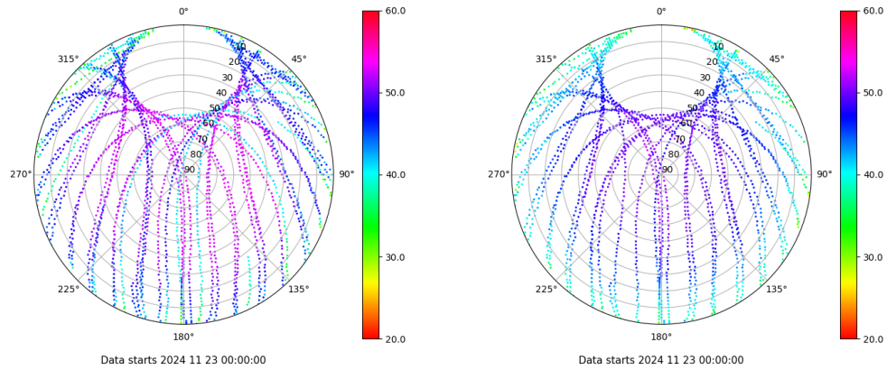
Skyplot for station ALBA. Signal to Noise S1C Data file ALBA00ESP_R_2024328.xtr Skyplot for station ALBA. Signal to Noise S2C Data file ALBA00ESP_R_2024328.xtr
