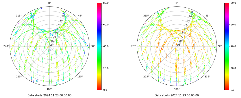
Skyplot for station ALBA. Parameter M1C Data file ALBA00ESP_R_2024328.xtr Skyplot for station ALBA. Parameter M2C Data file ALBA00ESP_R_2024328.xtr
