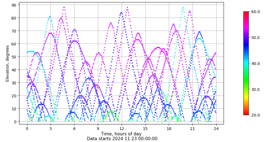
Time-elevation plot for station ALBA. Signal to Noise S1C Data file ALBA00ESP_R_2024328.xtr
