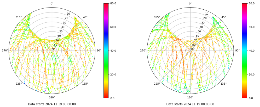
Skyplot for station ALBA. Parameter M1C Data file ALBA00ESP_R_2024324.xtr Skyplot for station ALBA. Parameter M2S Data file ALBA00ESP_R_2024324.xtr
