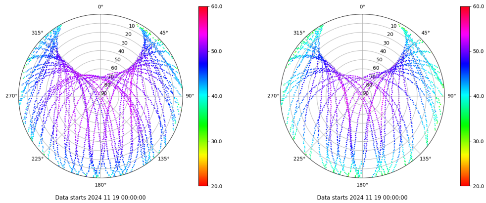
Skyplot for station ALBA. Signal to Noise S1C Data file ALBA00ESP_R_2024324.xtr Skyplot for station ALBA. Signal to Noise S2S Data file ALBA00ESP_R_2024324.xtr
