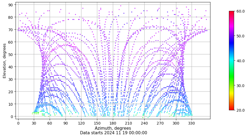
Azimuth-elevation plot for station ALBA. Signal to Noise S1C Data file ALBA00ESP_R_2024324.xtr
