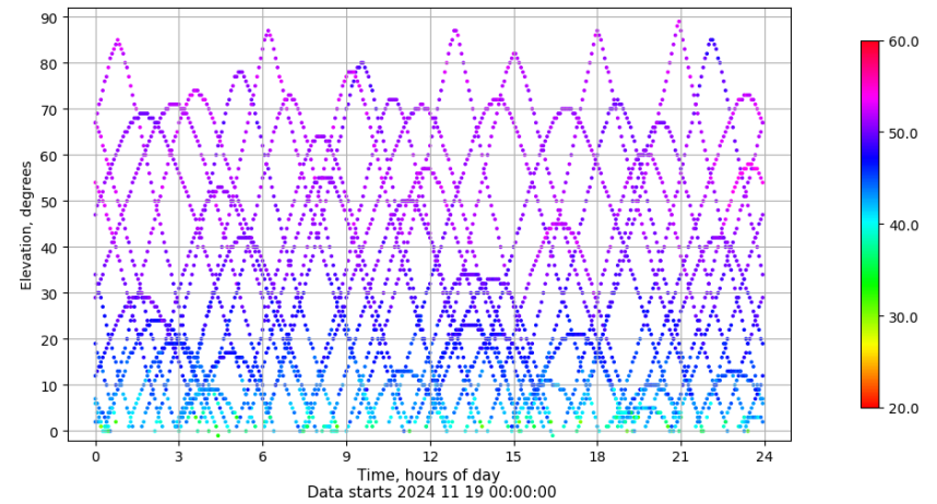
Time-elevation plot for station ALBA. Signal to Noise S1C Data file ALBA00ESP_R_2024324.xtr
