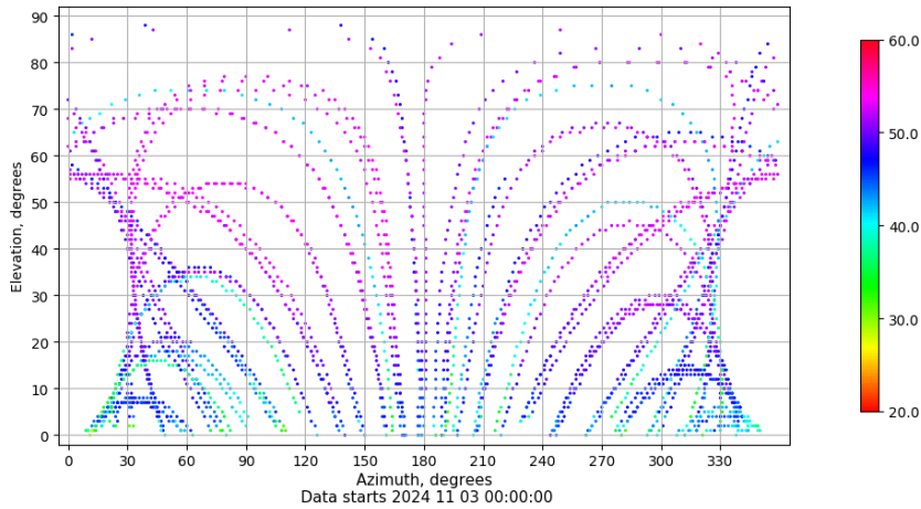
Azimuth-elevation plot for station ALBA. Signal to Noise S1C Data file ALBA00ESP_R_2024308.xtr
