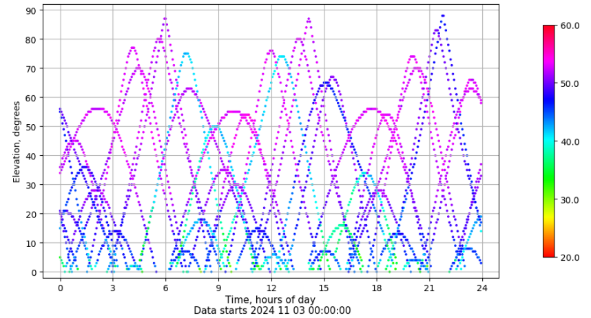
Time-elevation plot for station ALBA. Signal to Noise S1C Data file ALBA00ESP_R_2024308.xtr
