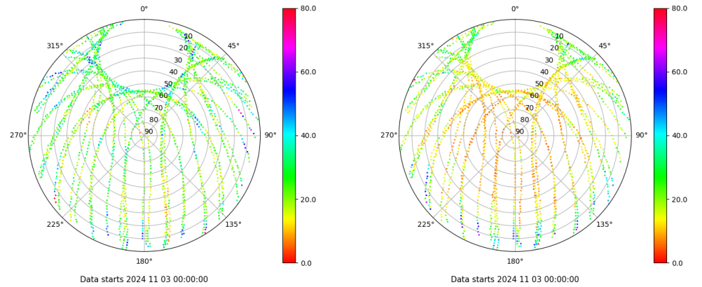
Skyplot for station ALBA. Parameter M1C Data file ALBA00ESP_R_2024308.xtr Skyplot for station ALBA. Parameter M2C Data file ALBA00ESP_R_2024308.xtr
