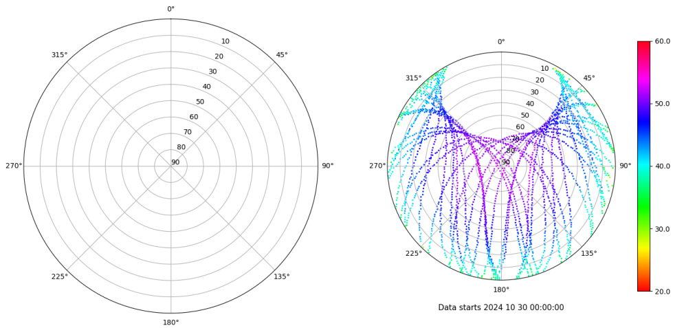
Skyplot for station ALBA. Signal to Noise S1C Data file ALBA00ESP_R_2024304.xtr Skyplot for station ALBA. Signal to Noise S2S Data file ALBA00ESP_R_2024304.xtr
