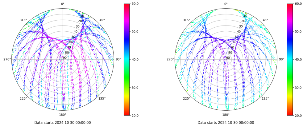
Skyplot for station ALBA. Signal to Noise S1C Data file ALBA00ESP_R_2024304.xtr Skyplot for station ALBA. Signal to Noise S2C Data file ALBA00ESP_R_2024304.xtr
