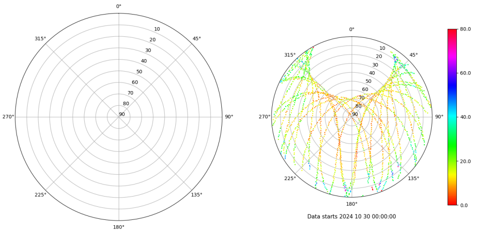
Skyplot for station ALBA. Parameter M1C Data file ALBA00ESP_R_2024304.xtr Skyplot for station ALBA. Parameter M2S Data file ALBA00ESP_R_2024304.xtr
