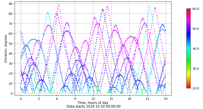
Time-elevation plot for station ALBA. Signal to Noise S1C Data file ALBA00ESP_R_2024304.xtr
