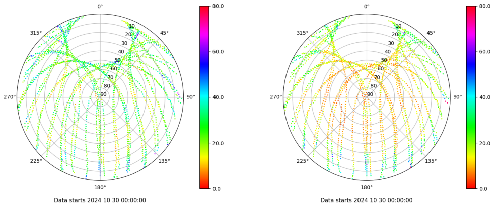
Skyplot for station ALBA. Parameter M1C Data file ALBA00ESP_R_2024304.xtr Skyplot for station ALBA. Parameter M2C Data file ALBA00ESP_R_2024304.xtr
