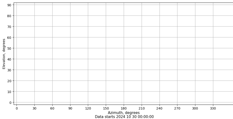
Azimuth-elevation plot for station ALBA. Signal to Noise S1C Data file ALBA00ESP_R_2024304.xtr
