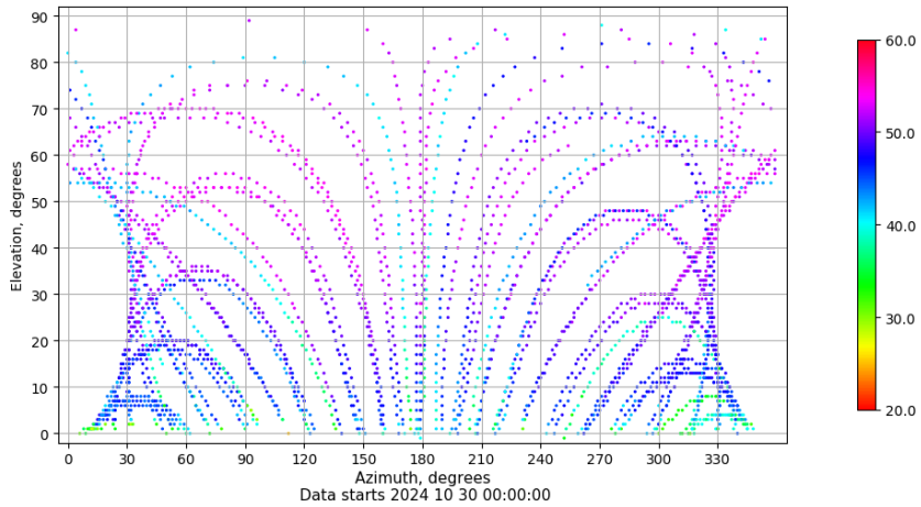
Azimuth-elevation plot for station ALBA. Signal to Noise S1C Data file ALBA00ESP_R_2024304.xtr
