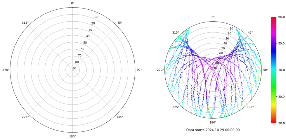
Skyplot for station ALBA. Signal to Noise S1C Data file ALBA00ESP_R_2024303.xtr Skyplot for station ALBA. Signal to Noise S2S Data file ALBA00ESP_R_2024303.xtr
