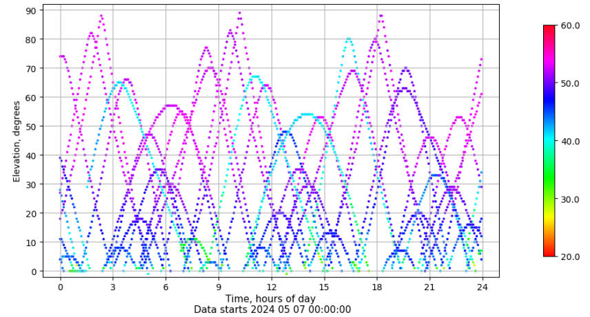
Time-elevation plot for station ALBA. Signal to Noise S1C Data file ALBA00ESP_R_2024128.xtr
