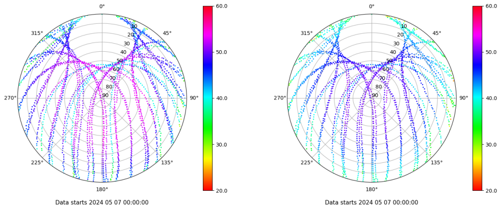
Skyplot for station ALBA. Signal to Noise S1C Data file ALBA00ESP_R_2024128.xtr Skyplot for station ALBA. Signal to Noise S2C Data file ALBA00ESP_R_2024128.xtr
