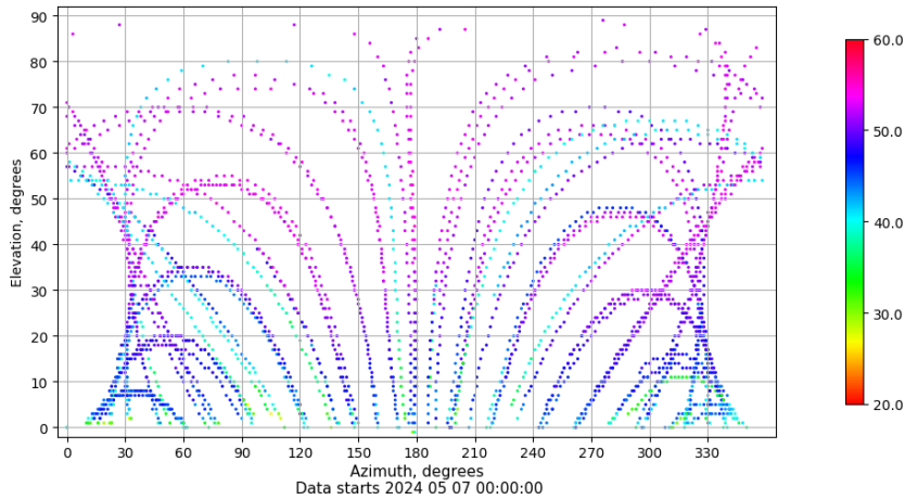
Azimuth-elevation plot for station ALBA. Signal to Noise S1C Data file ALBA00ESP_R_2024128.xtr
