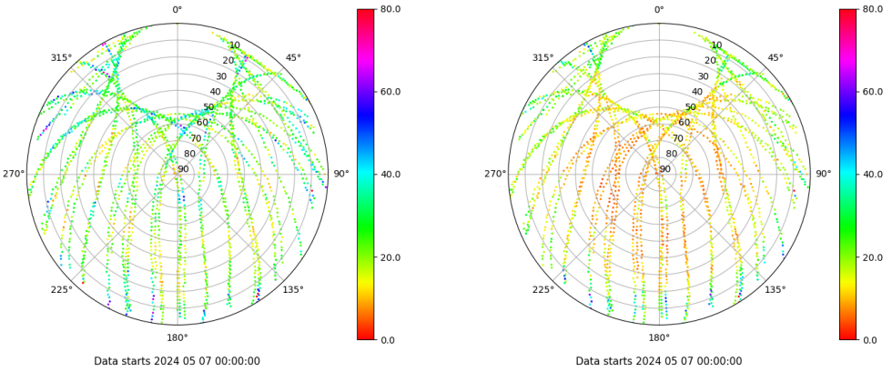
Skyplot for station ALBA. Parameter M1C Data file ALBA00ESP_R_2024128.xtr Skyplot for station ALBA. Parameter M2C Data file ALBA00ESP_R_2024128.xtr
