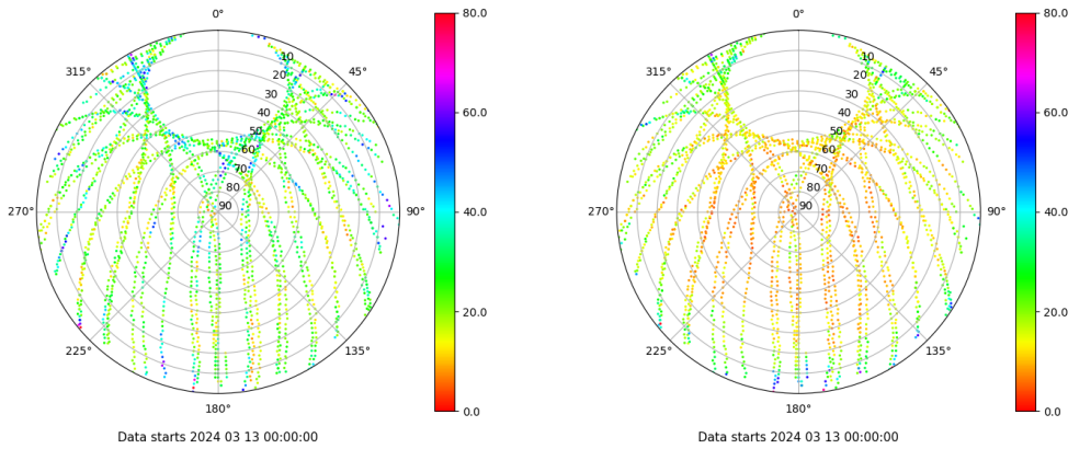
Skyplot for station ALBA. Parameter M1C Data file ALBA00ESP_R_2024073.xtr Skyplot for station ALBA. Parameter M2C Data file ALBA00ESP_R_2024073.xtr
