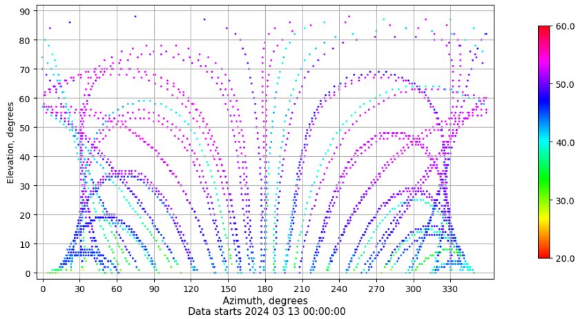
Azimuth-elevation plot for station ALBA. Signal to Noise S1C Data file ALBA00ESP_R_2024073.xtr
