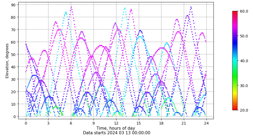
Time-elevation plot for station ALBA. Signal to Noise S1C Data file ALBA00ESP_R_2024073.xtr
