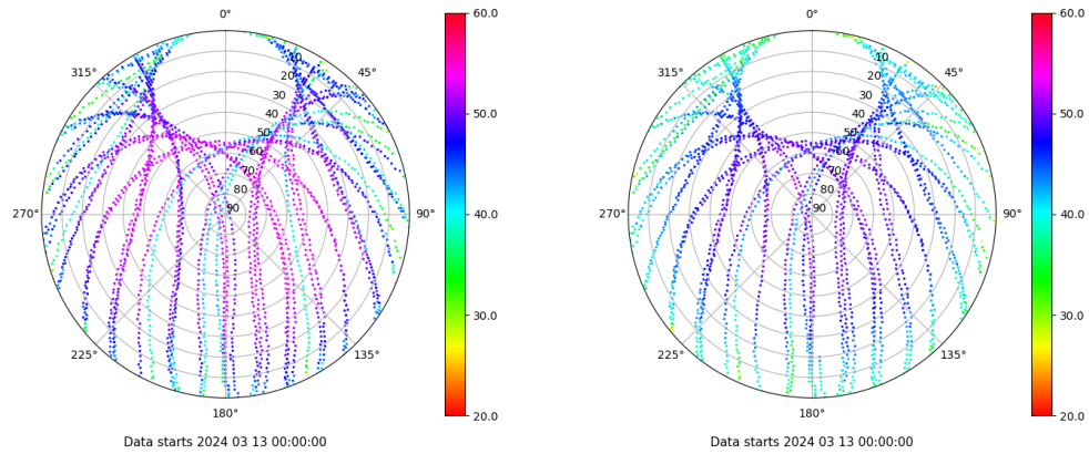
Skyplot for station ALBA. Signal to Noise S1C Data file ALBA00ESP_R_2024073.xtr Skyplot for station ALBA. Signal to Noise S2C Data file ALBA00ESP_R_2024073.xtr
