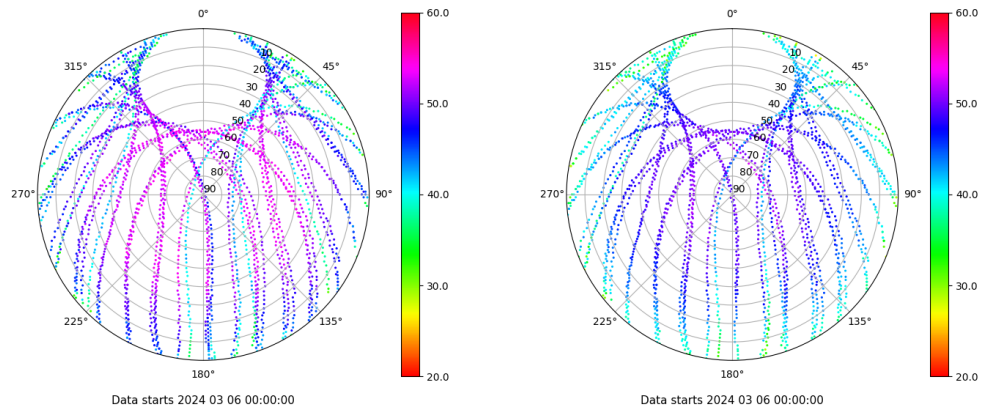
Skyplot for station ALBA. Signal to Noise S1C Data file ALBA00ESP_R_2024066.xtr Skyplot for station ALBA. Signal to Noise S2C Data file ALBA00ESP_R_2024066.xtr
