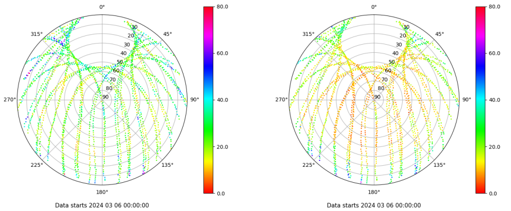
Skyplot for station ALBA. Parameter M1C Data file ALBA00ESP_R_2024066.xtr Skyplot for station ALBA. Parameter M2C Data file ALBA00ESP_R_2024066.xtr
