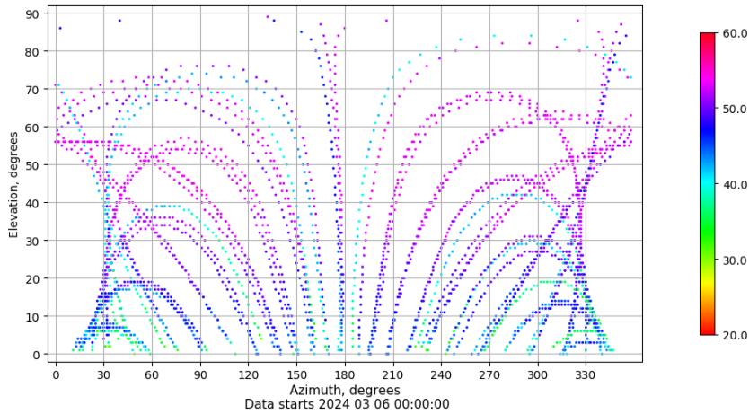
Azimuth-elevation plot for station ALBA. Signal to Noise S1C Data file ALBA00ESP_R_2024066.xtr
