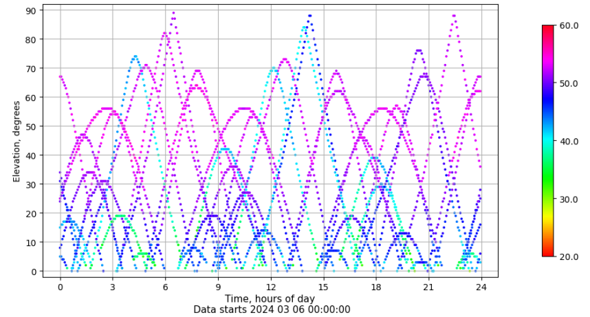
Time-elevation plot for station ALBA. Signal to Noise S1C Data file ALBA00ESP_R_2024066.xtr
