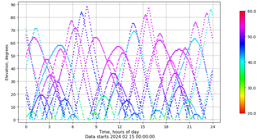
Time-elevation plot for station ALBA. Signal to Noise S1C Data file ALBA00ESP_R_2024046.xtr
