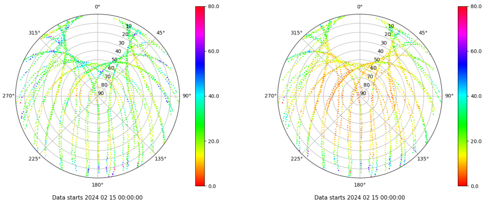
Skyplot for station ALBA. Parameter M1C Data file ALBA00ESP_R_2024046.xtr Skyplot for station ALBA. Parameter M2C Data file ALBA00ESP_R_2024046.xtr
