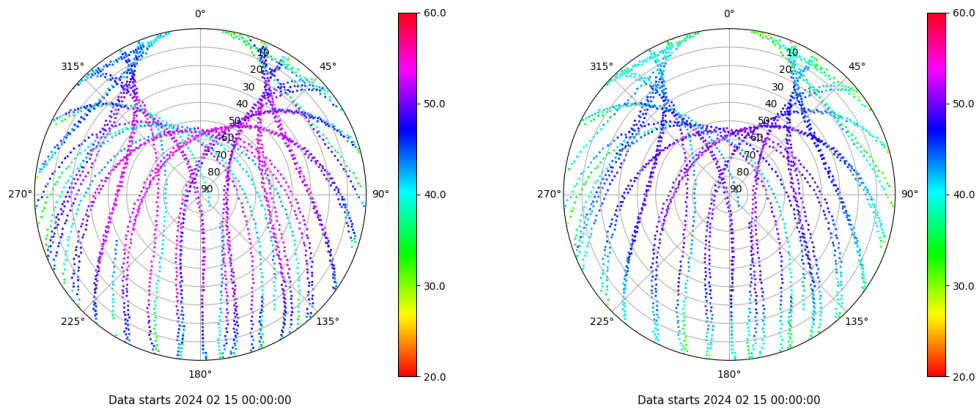
Skyplot for station ALBA. Signal to Noise S1C Data file ALBA00ESP_R_2024046.xtr Skyplot for station ALBA. Signal to Noise S2C Data file ALBA00ESP_R_2024046.xtr
