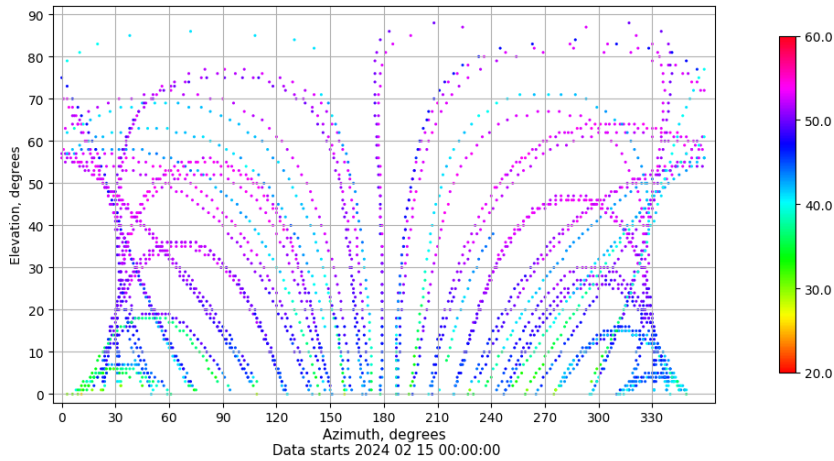
Azimuth-elevation plot for station ALBA. Signal to Noise S1C Data file ALBA00ESP_R_2024046.xtr
