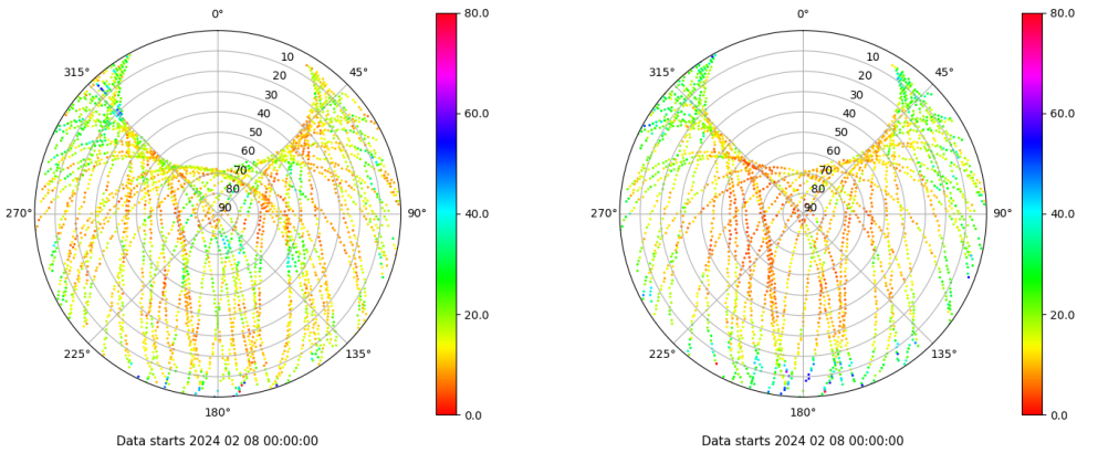
Skyplot for station ALBA. Parameter M1C Data file ALBA00ESP_R_2024039.xtr Skyplot for station ALBA. Parameter M2S Data file ALBA00ESP_R_2024039.xtr
