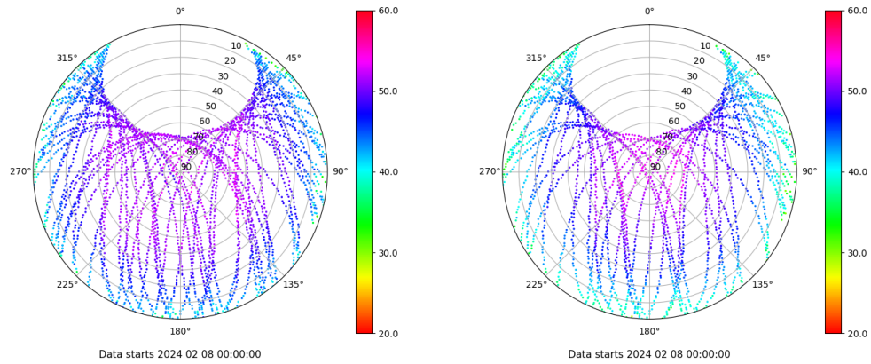
Skyplot for station ALBA. Signal to Noise S1C Data file ALBA00ESP_R_2024039.xtr Skyplot for station ALBA. Signal to Noise S2S Data file ALBA00ESP_R_2024039.xtr
