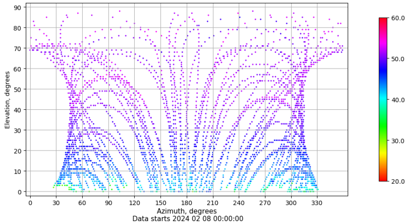
Azimuth-elevation plot for station ALBA. Signal to Noise S1C Data file ALBA00ESP_R_2024039.xtr
