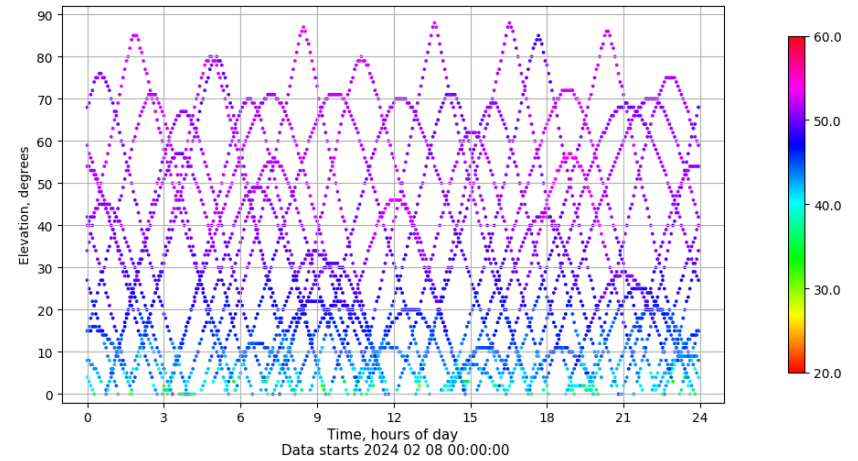
Time-elevation plot for station ALBA. Signal to Noise S1C Data file ALBA00ESP_R_2024039.xtr
