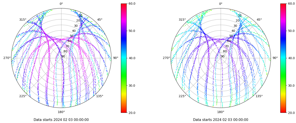
Skyplot for station ALBA. Signal to Noise S1C Data file ALBA00ESP_R_2024034.xtr Skyplot for station ALBA. Signal to Noise S2C Data file ALBA00ESP_R_2024034.xtr
