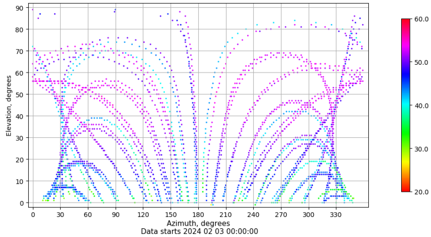
Azimuth-elevation plot for station ALBA. Signal to Noise S1C Data file ALBA00ESP_R_2024034.xtr
