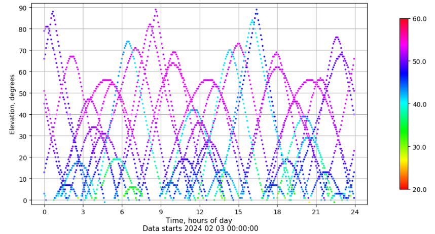
Time-elevation plot for station ALBA. Signal to Noise S1C Data file ALBA00ESP_R_2024034.xtr
