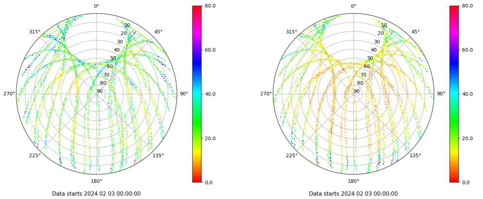
Skyplot for station ALBA. Parameter M1C Data file ALBA00ESP_R_2024034.xtr Skyplot for station ALBA. Parameter M2C Data file ALBA00ESP_R_2024034.xtr
