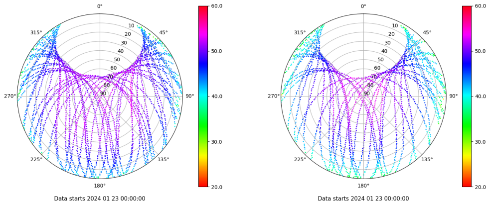
Skyplot for station ALBA. Signal to Noise S1C Data file ALBA00ESP_R_2024023.xtr Skyplot for station ALBA. Signal to Noise S2S Data file ALBA00ESP_R_2024023.xtr
