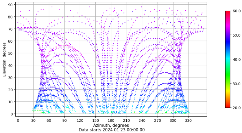
Azimuth-elevation plot for station ALBA. Signal to Noise S1C Data file ALBA00ESP_R_2024023.xtr
