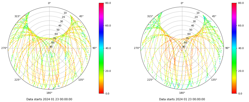
Skyplot for station ALBA. Parameter M1C Data file ALBA00ESP_R_2024023.xtr Skyplot for station ALBA. Parameter M2S Data file ALBA00ESP_R_2024023.xtr
