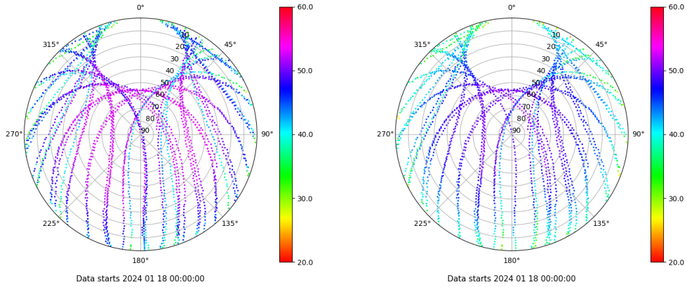
Skyplot for station ALBA. Signal to Noise S1C Data file ALBA00ESP_R_2024018.xtr Skyplot for station ALBA. Signal to Noise S2C Data file ALBA00ESP_R_2024018.xtr
