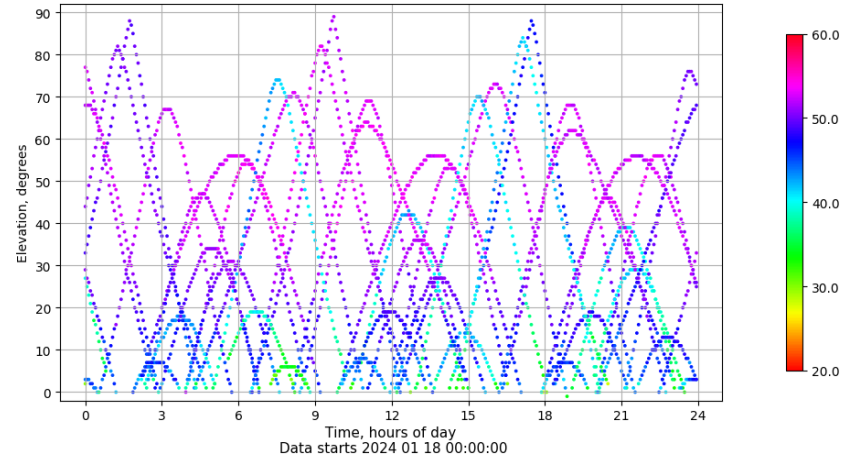
Time-elevation plot for station ALBA. Signal to Noise S1C Data file ALBA00ESP_R_2024018.xtr
