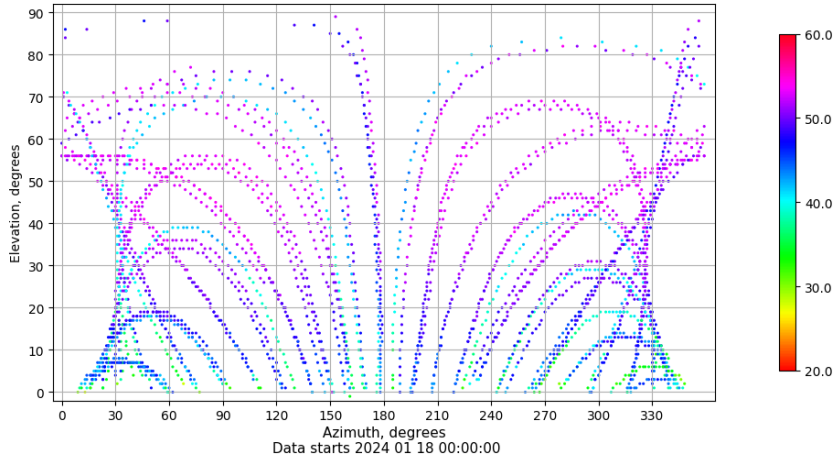
Azimuth-elevation plot for station ALBA. Signal to Noise S1C Data file ALBA00ESP_R_2024018.xtr
