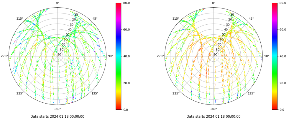
Skyplot for station ALBA. Parameter M1C Data file ALBA00ESP_R_2024018.xtr Skyplot for station ALBA. Parameter M2C Data file ALBA00ESP_R_2024018.xtr
