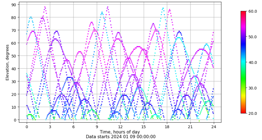
Time-elevation plot for station ALBA. Signal to Noise S1C Data file ALBA00ESP_R_2024009.xtr
