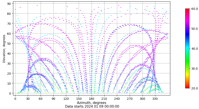
Azimuth-elevation plot for station ALBA. Signal to Noise S1C Data file ALBA00ESP_R_2024009.xtr
