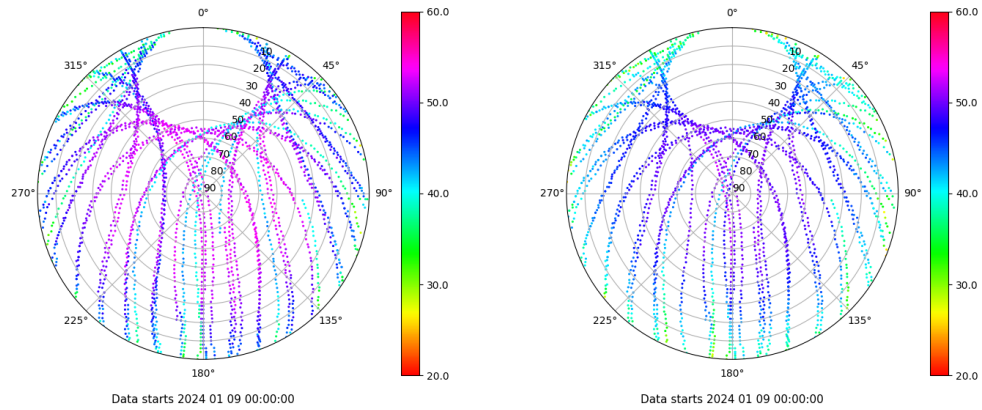
Skyplot for station ALBA. Signal to Noise S1C Data file ALBA00ESP_R_2024009.xtr Skyplot for station ALBA. Signal to Noise S2C Data file ALBA00ESP_R_2024009.xtr
