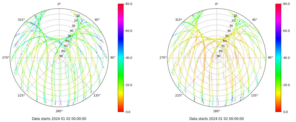
Skyplot for station ALBA. Parameter M1C Data file ALBA00ESP_R_2024002.xtr Skyplot for station ALBA. Parameter M2C Data file ALBA00ESP_R_2024002.xtr
