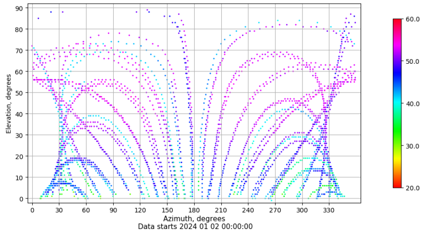
Azimuth-elevation plot for station ALBA. Signal to Noise S1C Data file ALBA00ESP_R_2024002.xtr
