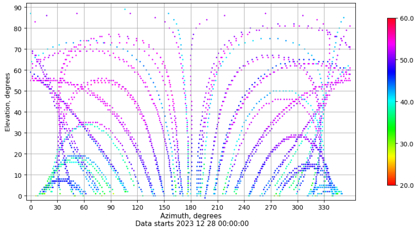
Azimuth-elevation plot for station ALBA. Signal to Noise S1C Data file ALBA00ESP_R_2023362.xtr
