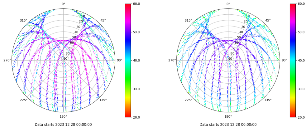
Skyplot for station ALBA. Signal to Noise S1C Data file ALBA00ESP_R_2023362.xtr Skyplot for station ALBA. Signal to Noise S2C Data file ALBA00ESP_R_2023362.xtr
