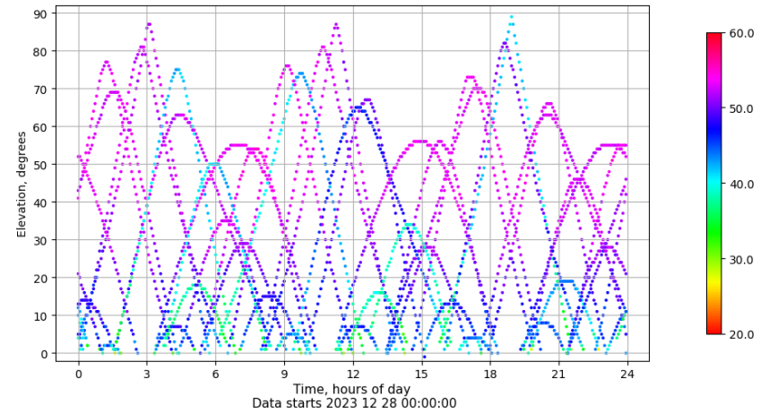
Time-elevation plot for station ALBA. Signal to Noise S1C Data file ALBA00ESP_R_2023362.xtr
