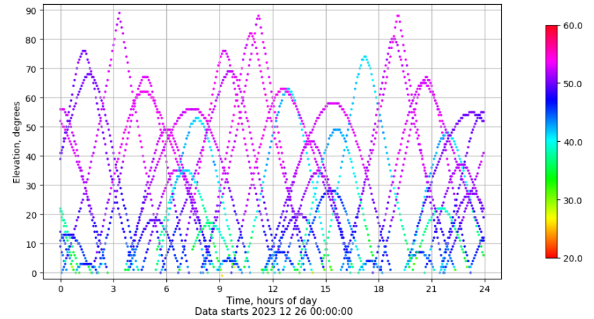
Time-elevation plot for station ALBA. Signal to Noise S1C Data file ALBA00ESP_R_2023360.xtr
