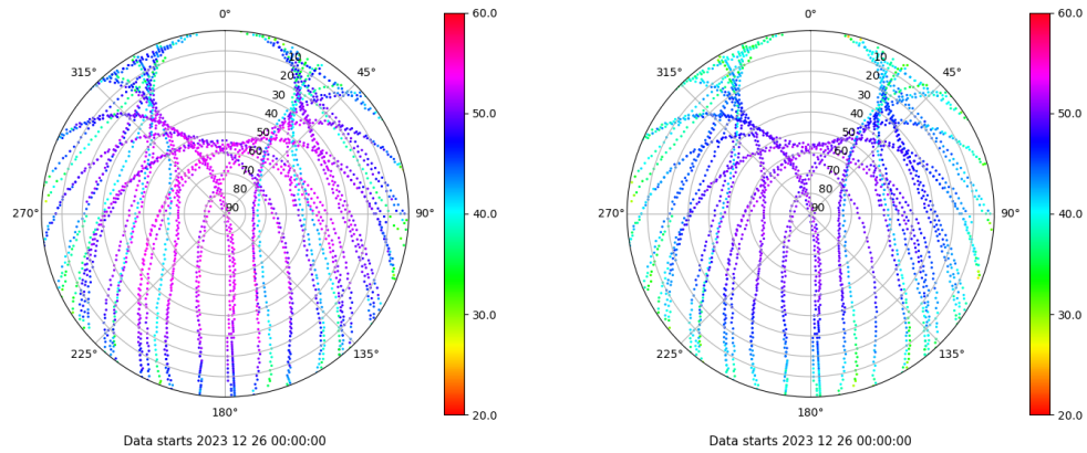
Skyplot for station ALBA. Signal to Noise S1C Data file ALBA00ESP_R_2023360.xtr Skyplot for station ALBA. Signal to Noise S2C Data file ALBA00ESP_R_2023360.xtr
