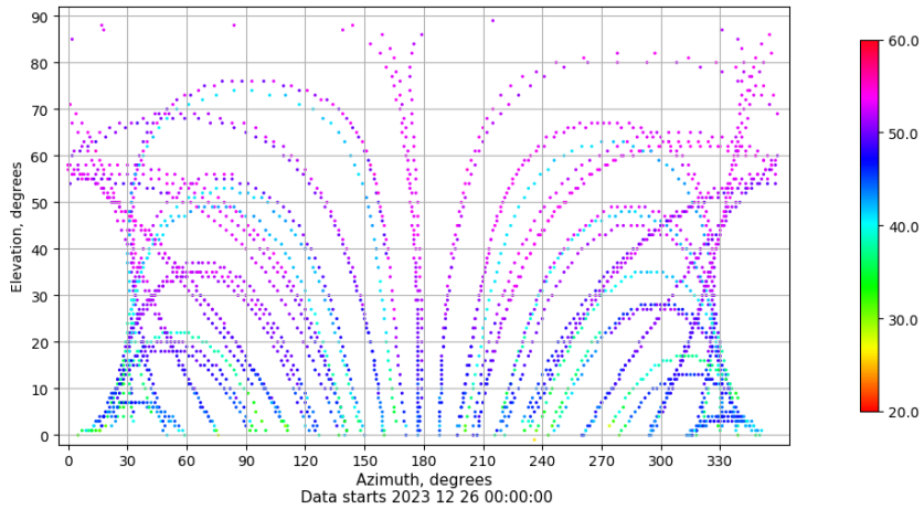
Azimuth-elevation plot for station ALBA. Signal to Noise S1C Data file ALBA00ESP_R_2023360.xtr
