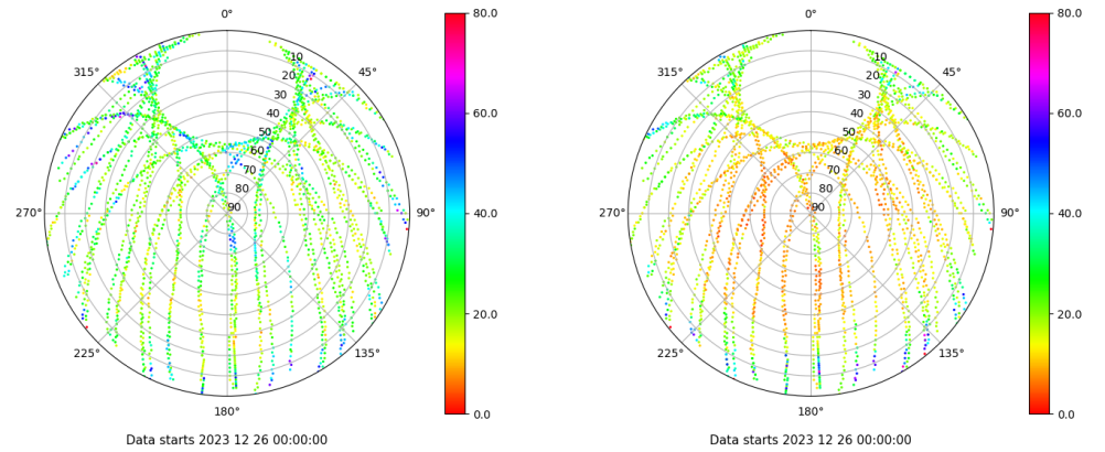
Skyplot for station ALBA. Parameter M1C Data file ALBA00ESP_R_2023360.xtr Skyplot for station ALBA. Parameter M2C Data file ALBA00ESP_R_2023360.xtr
