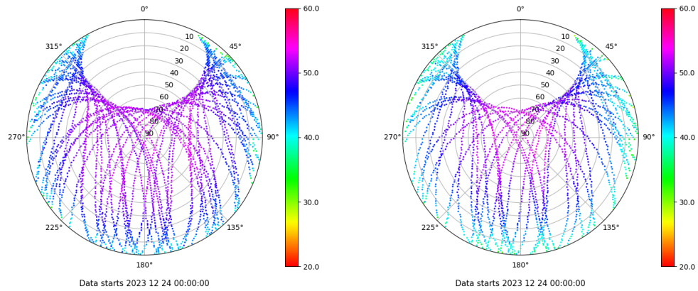
Skyplot for station ALBA. Signal to Noise S1C Data file ALBA00ESP_R_2023358.xtr Skyplot for station ALBA. Signal to Noise S2S Data file ALBA00ESP_R_2023358.xtr
