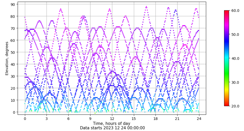
Time-elevation plot for station ALBA. Signal to Noise S1C Data file ALBA00ESP_R_2023358.xtr
