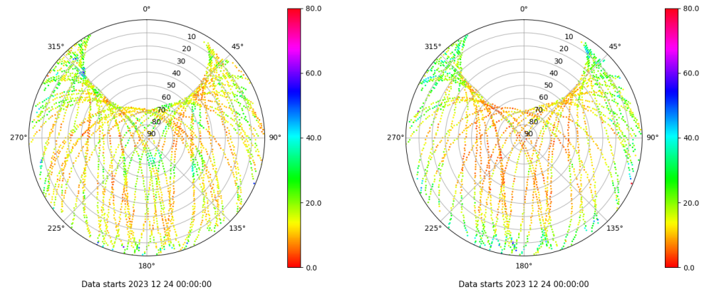
Skyplot for station ALBA. Parameter M1C Data file ALBA00ESP_R_2023358.xtr Skyplot for station ALBA. Parameter M2S Data file ALBA00ESP_R_2023358.xtr
