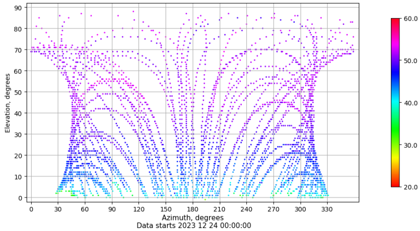
Azimuth-elevation plot for station ALBA. Signal to Noise S1C Data file ALBA00ESP_R_2023358.xtr
