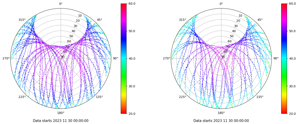
Skyplot for station ALBA. Signal to Noise S1C Data file ALBA00ESP_R_2023334.xtr Skyplot for station ALBA. Signal to Noise S2S Data file ALBA00ESP_R_2023334.xtr
