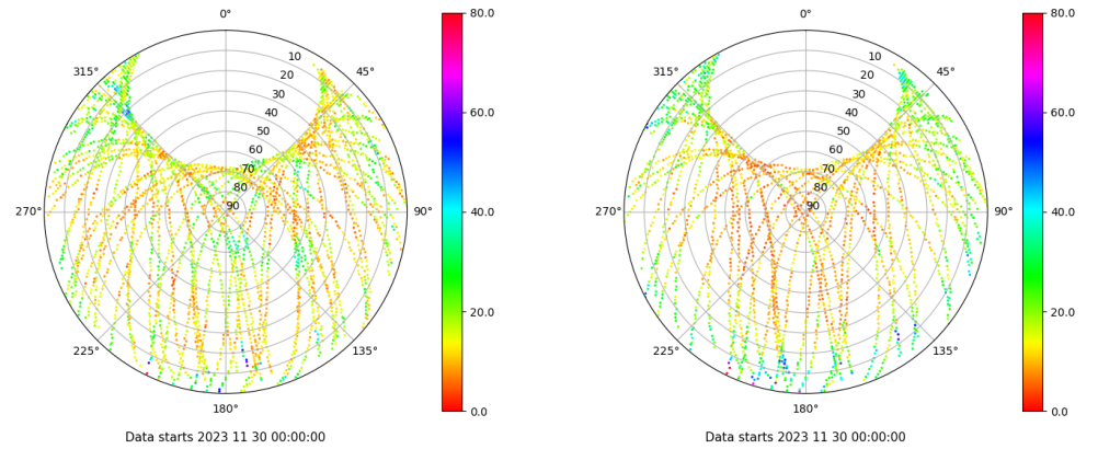
Skyplot for station ALBA. Parameter M1C Data file ALBA00ESP_R_2023334.xtr Skyplot for station ALBA. Parameter M2S Data file ALBA00ESP_R_2023334.xtr
