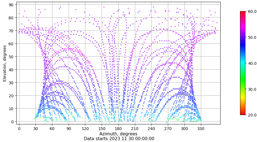
Azimuth-elevation plot for station ALBA. Signal to Noise S1C Data file ALBA00ESP_R_2023334.xtr
