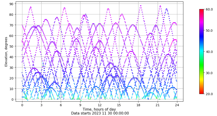
Time-elevation plot for station ALBA. Signal to Noise S1C Data file ALBA00ESP_R_2023334.xtr
