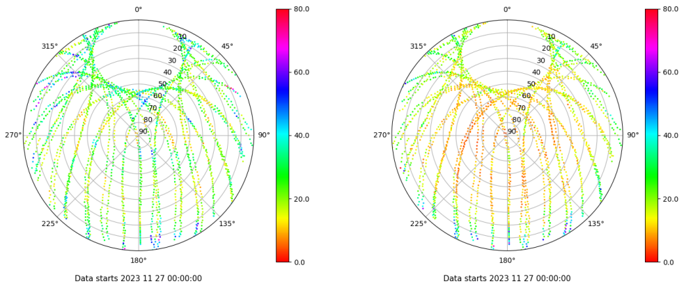
Skyplot for station ALBA. Parameter M1C Data file ALBA00ESP_R_2023331.xtr Skyplot for station ALBA. Parameter M2C Data file ALBA00ESP_R_2023331.xtr
