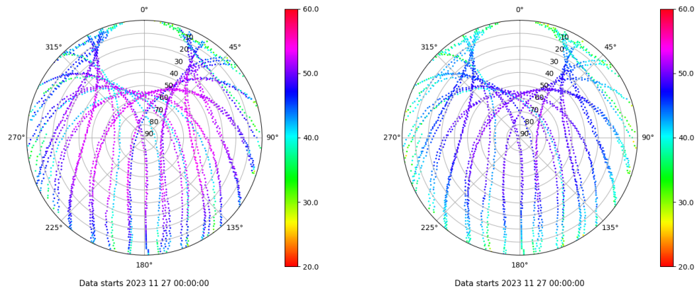
Skyplot for station ALBA. Signal to Noise S1C Data file ALBA00ESP_R_2023331.xtr Skyplot for station ALBA. Signal to Noise S2C Data file ALBA00ESP_R_2023331.xtr
