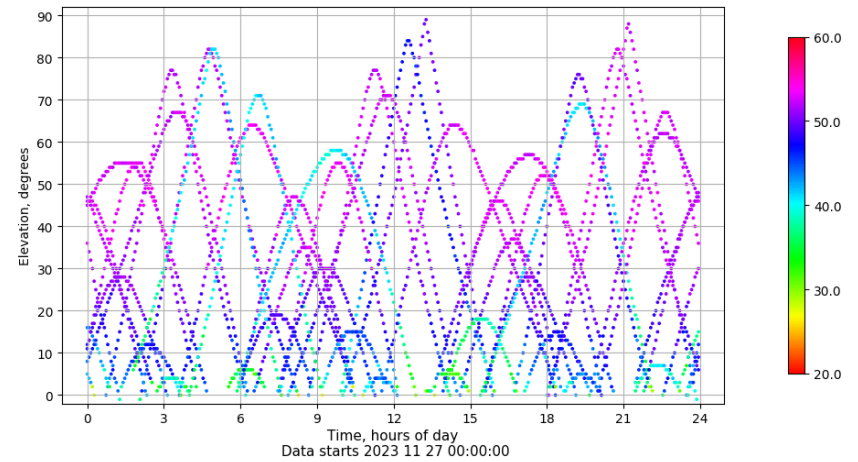
Time-elevation plot for station ALBA. Signal to Noise S1C Data file ALBA00ESP_R_2023331.xtr
