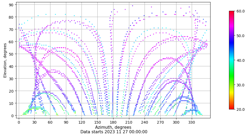
Azimuth-elevation plot for station ALBA. Signal to Noise S1C Data file ALBA00ESP_R_2023331.xtr
